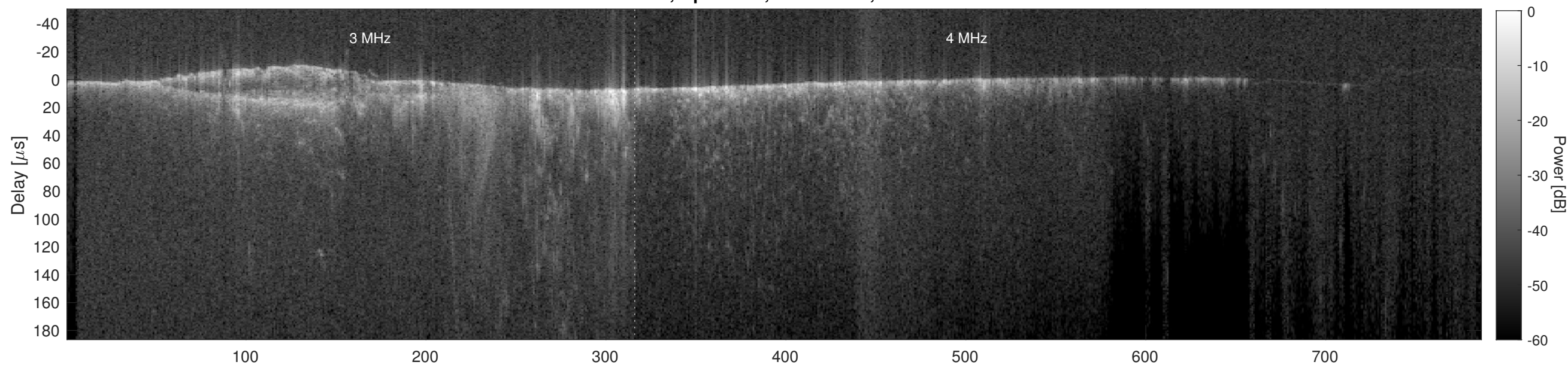
Orbit 9563, Cluttergram
