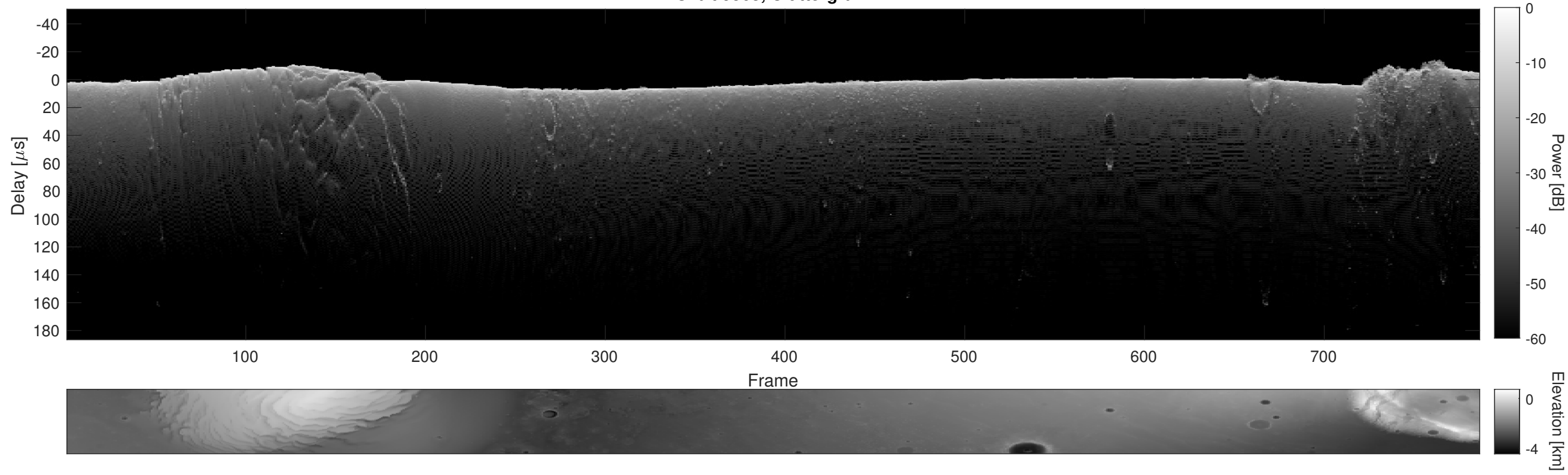
Orbit 9563, Cluttergram
