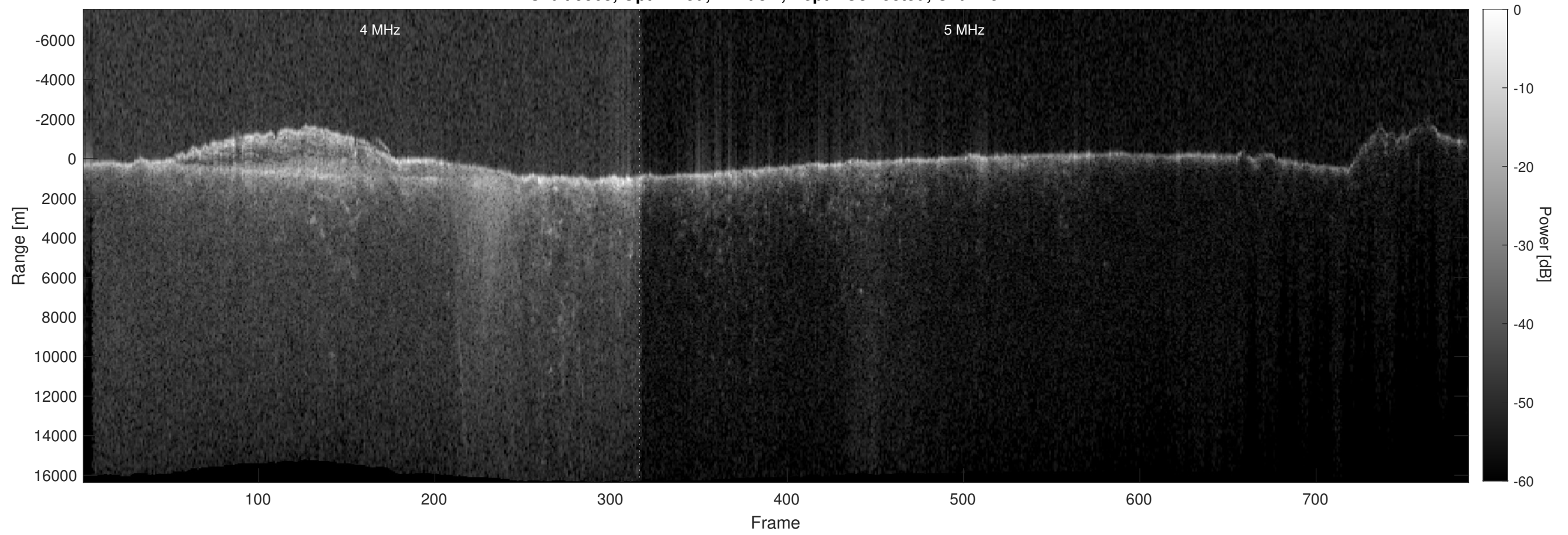
Orbit 9563, Optimized, Window, Depth-Corrected, Channel 2
