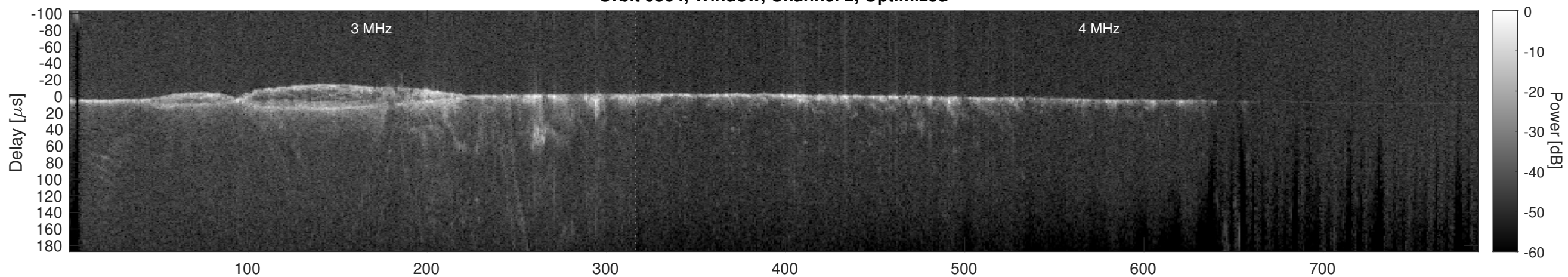
Orbit 9564, Cluttergram
