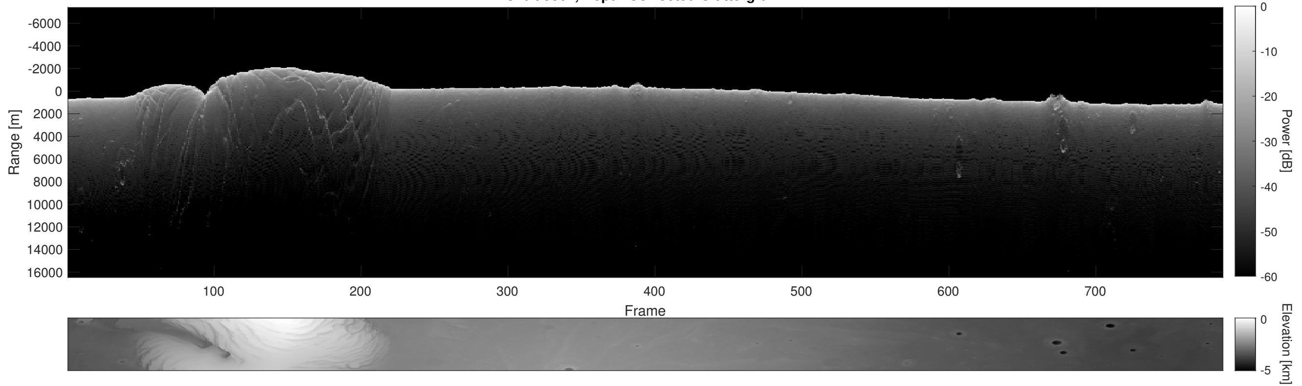
Orbit 9564, Depth-Corrected Cluttergram
