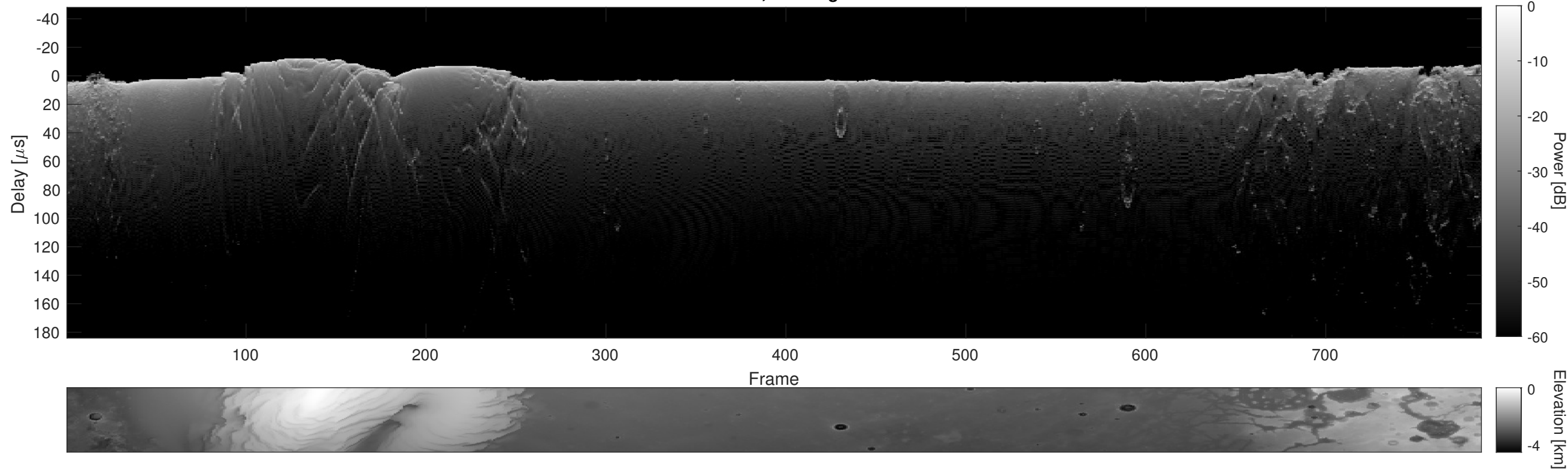
Orbit 9565, Cluttergram
