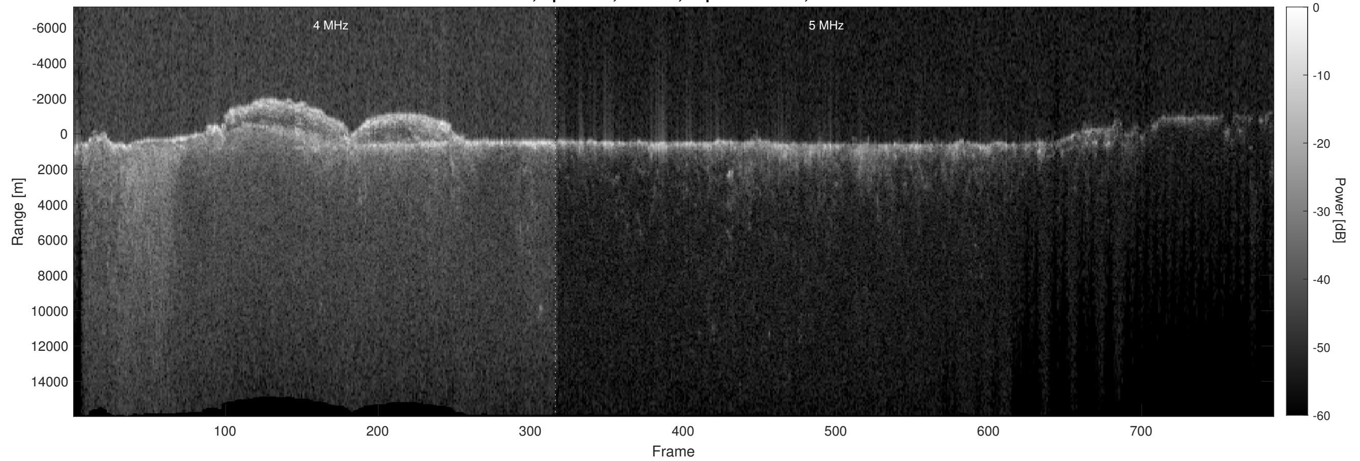
Orbit 9565, Optimized, Window, Depth-Corrected, Channel 2
