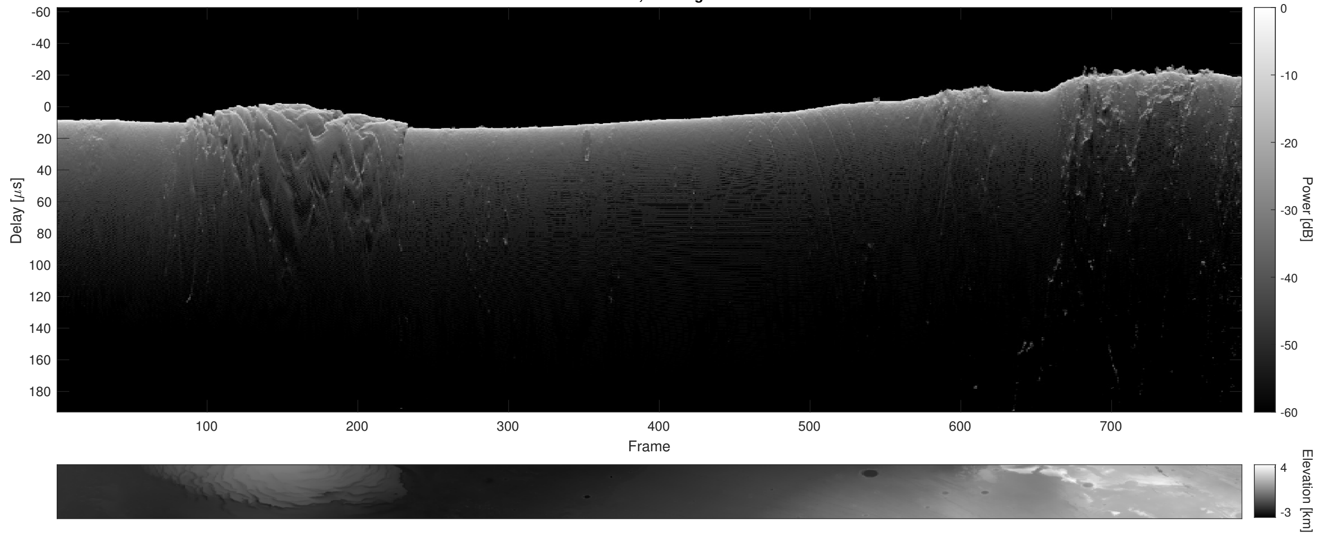
Orbit 9566, Cluttergram
