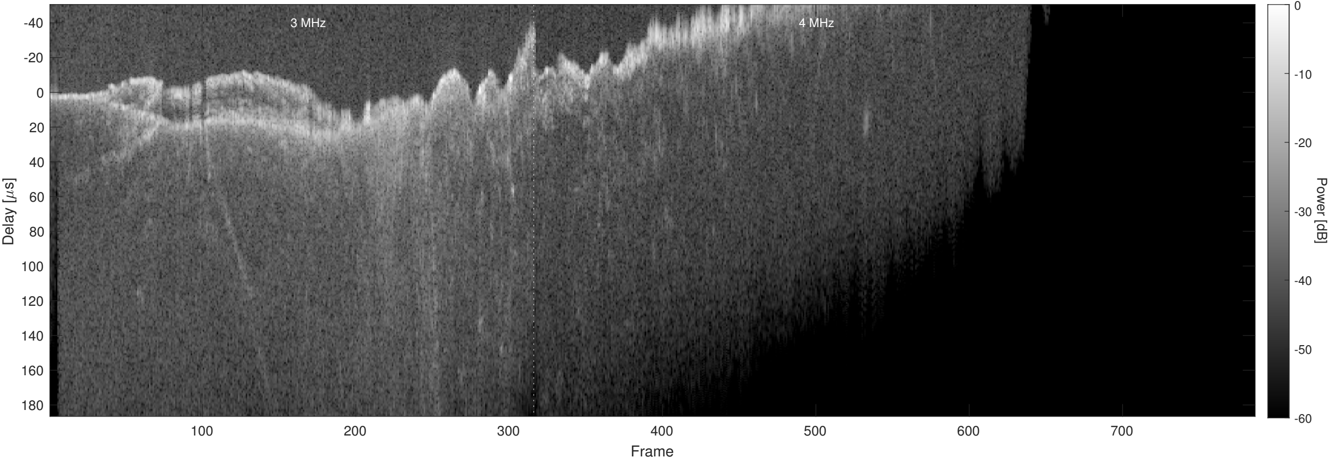
Orbit 9567, Chapman, Window, Channel 2
