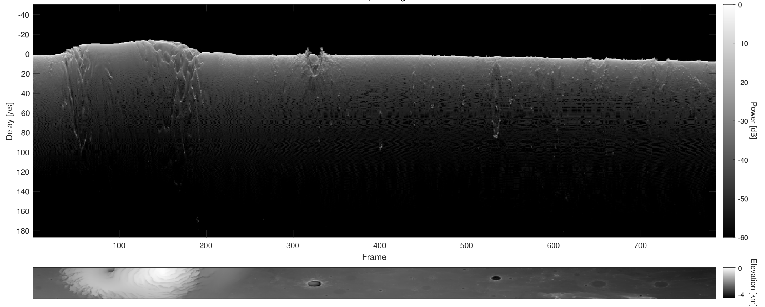
Orbit 9567, Cluttergram
