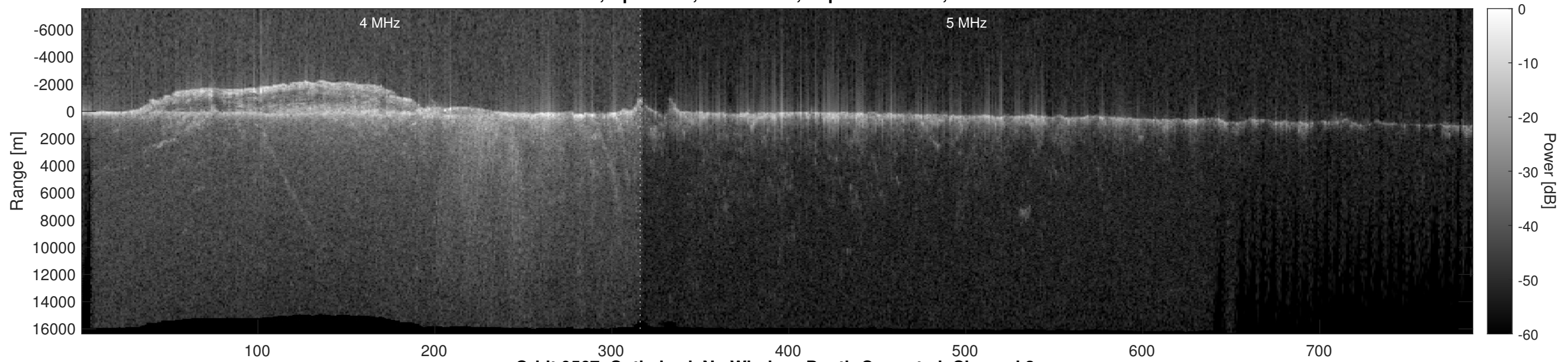
Orbit 9567, Optimized, No Window, Depth-Corrected, Channel 2
