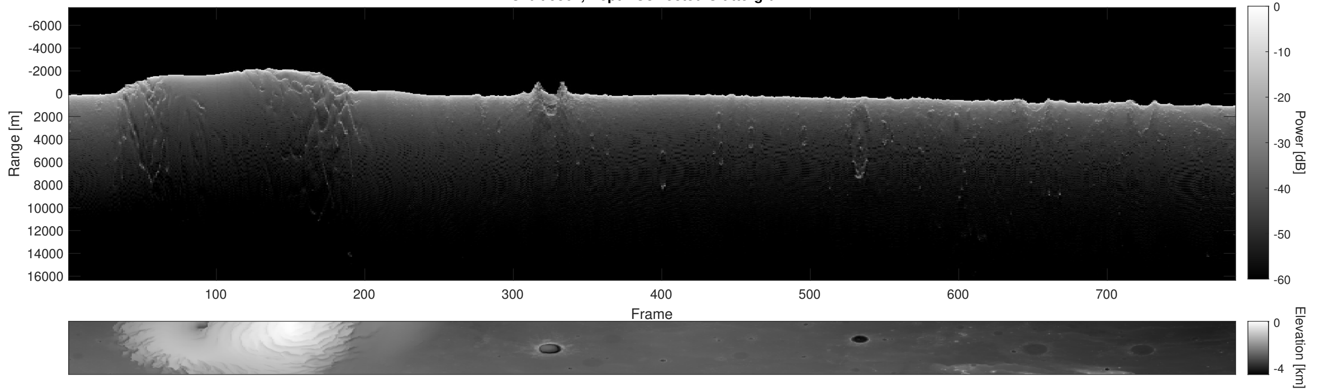
Orbit 9567, Depth-Corrected Cluttergram
