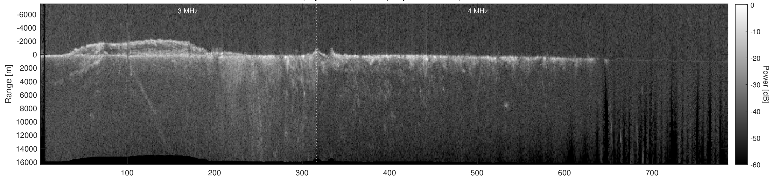
Orbit 9567, Depth-Corrected Cluttergram
