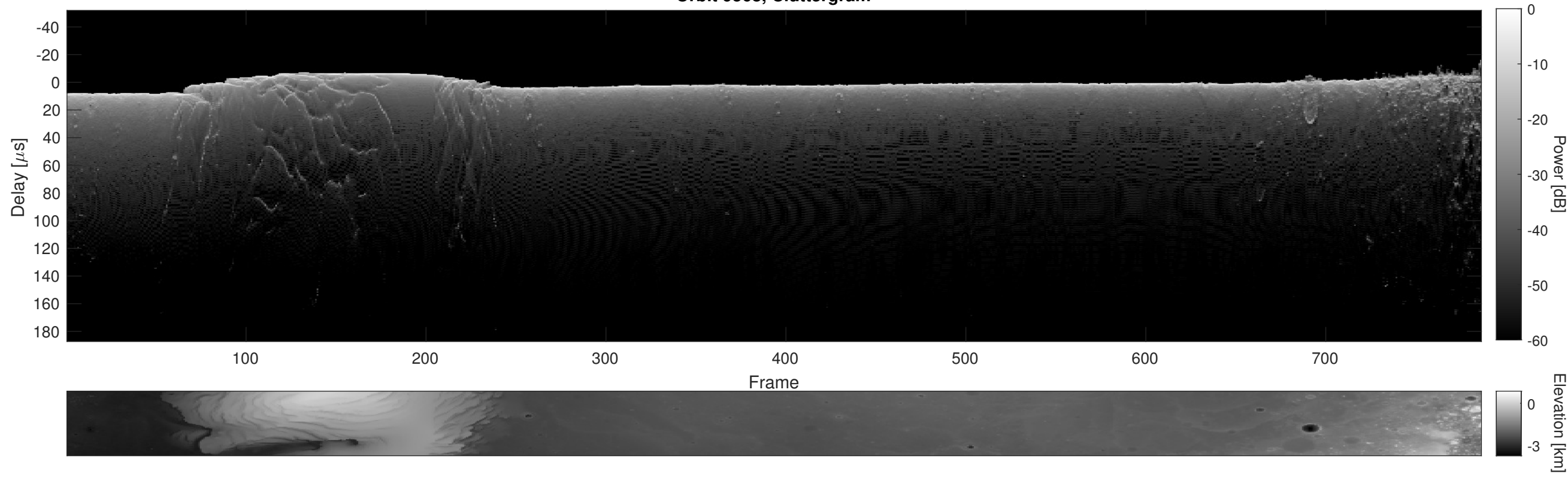
Orbit 9568, Cluttergram
