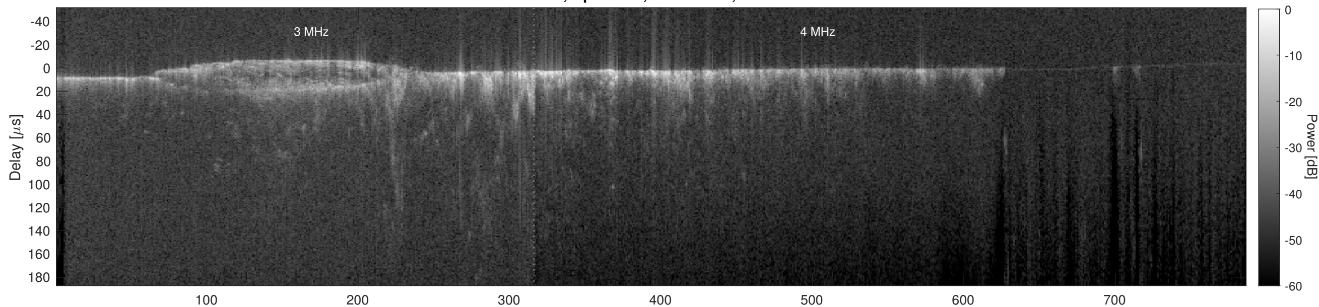
Orbit 9568, Cluttergram
