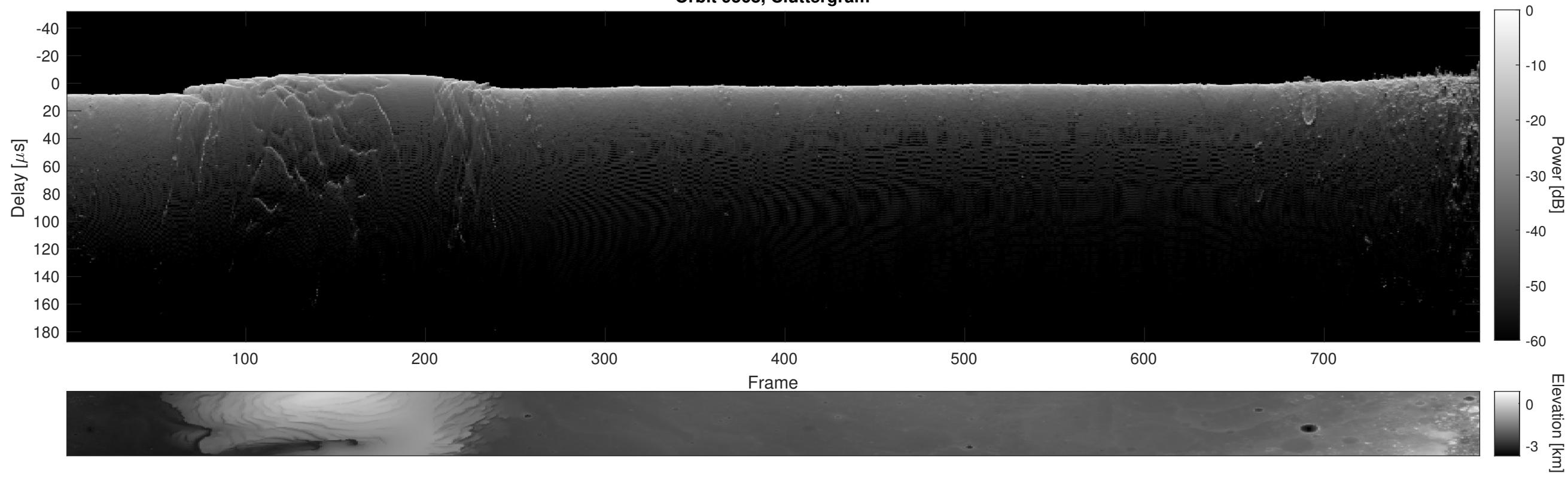
Orbit 9568, Cluttergram
