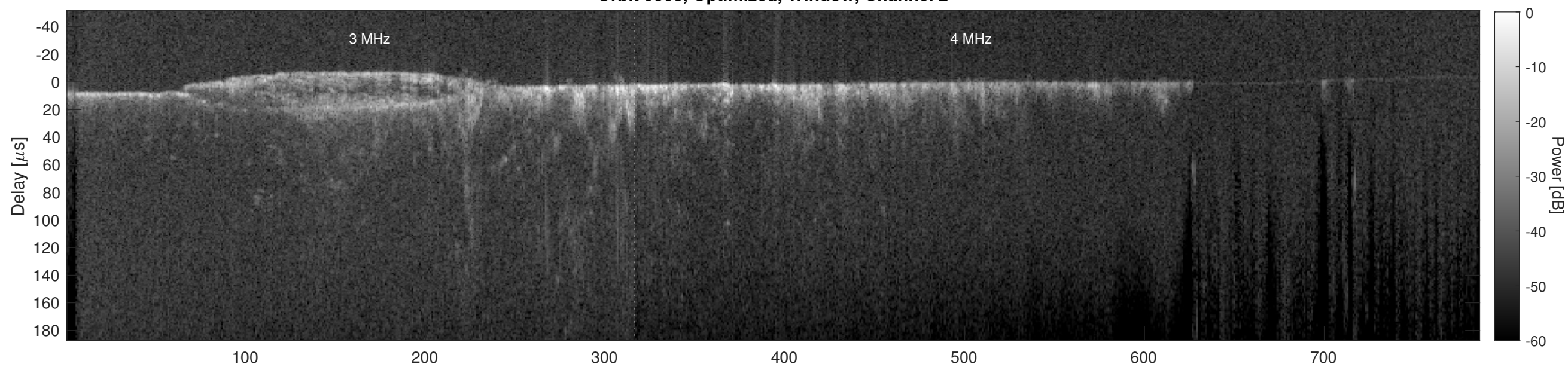
Orbit 9568, Cluttergram
