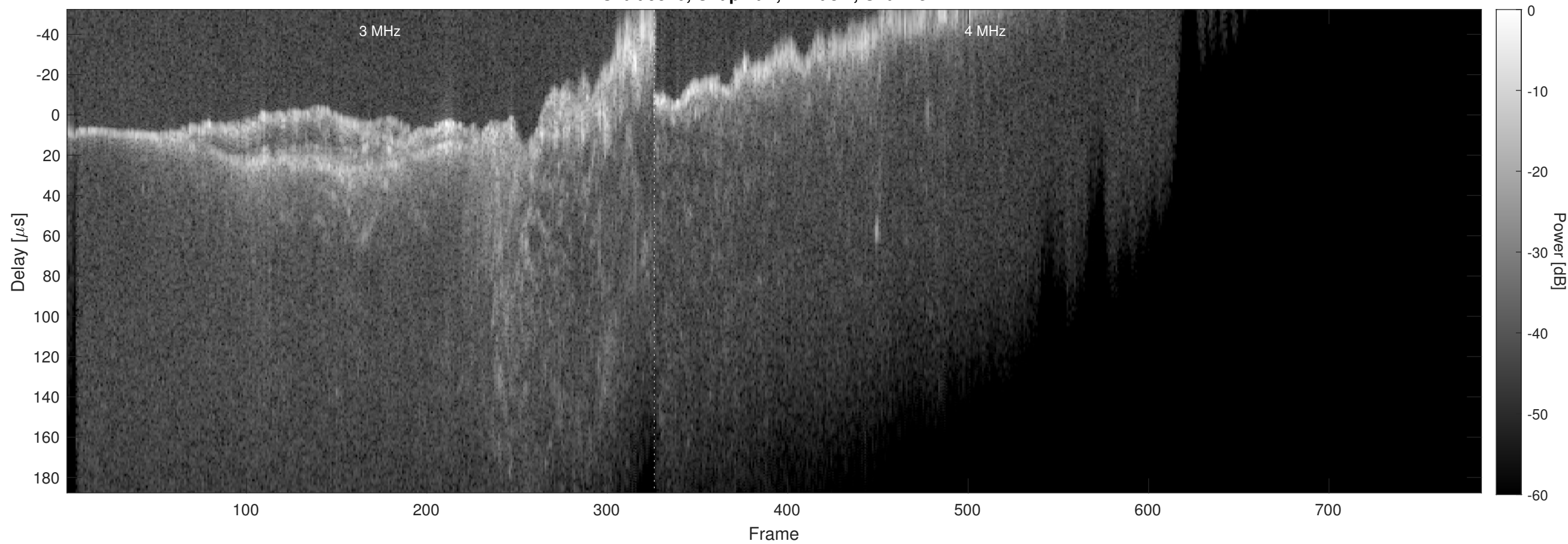
Orbit 9570, Chapman, Window, Channel 2
