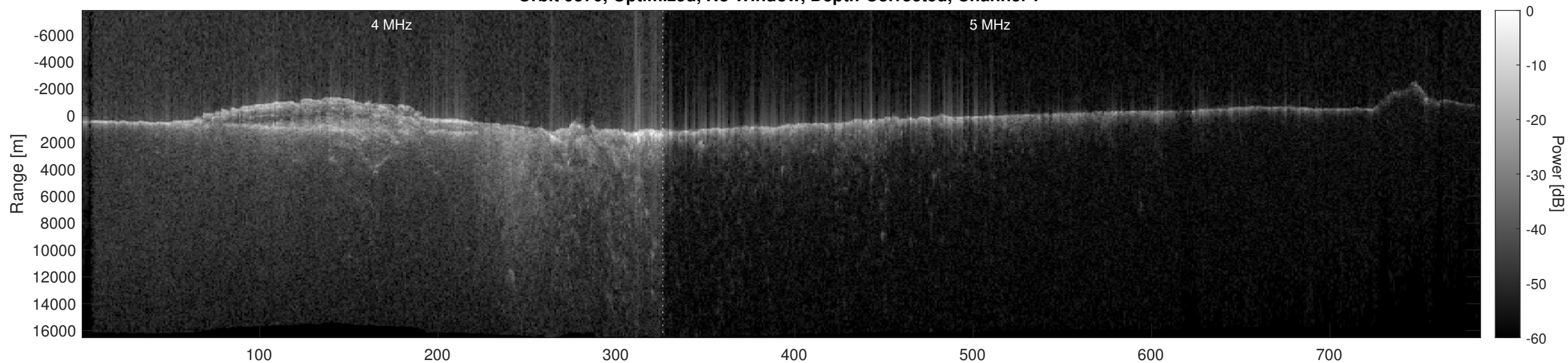
Orbit 9570, Optimized, No Window, Depth-Corrected, Channel 2
