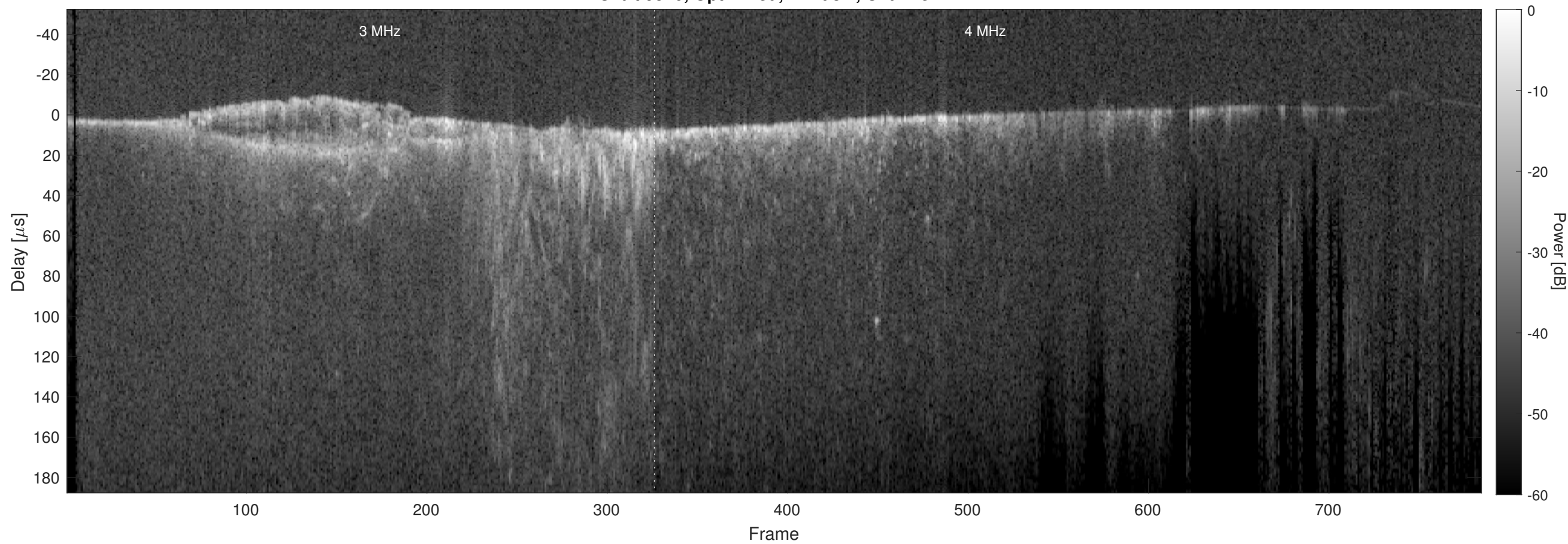
Orbit 9570, Optimized, Window, Channel 2
