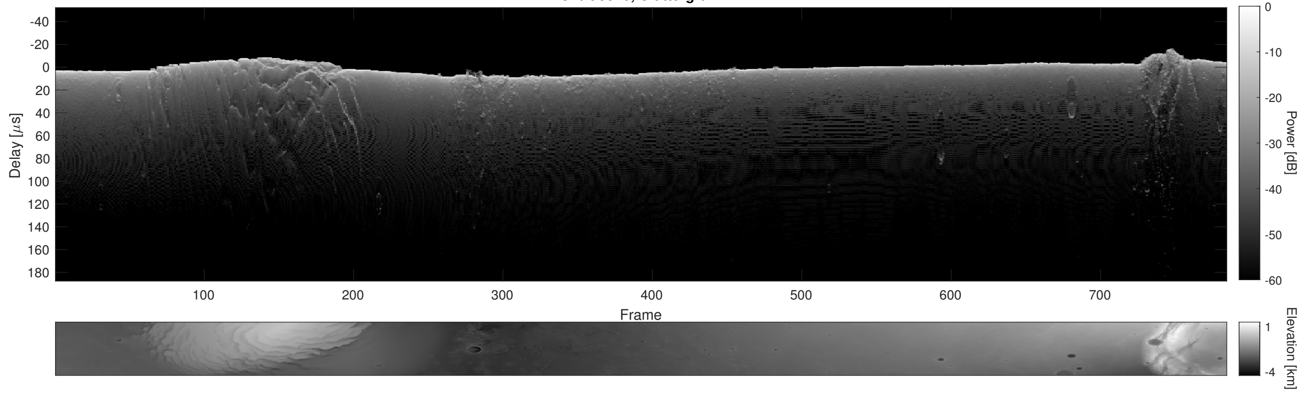
Orbit 9570, Cluttergram
