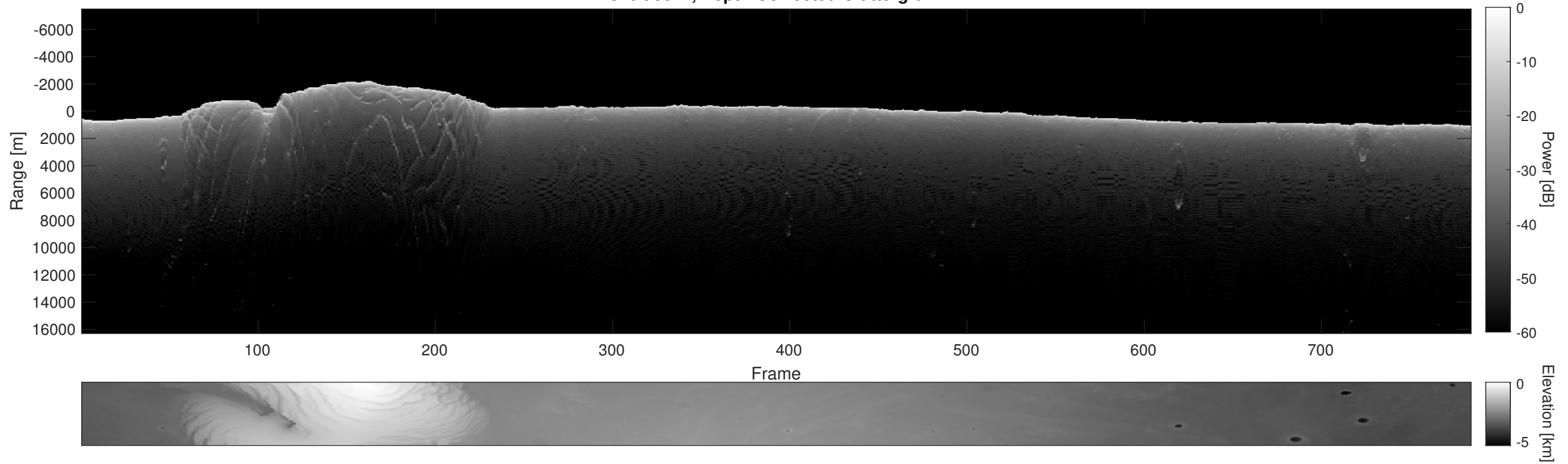
Orbit 9571, Depth-Corrected Cluttergram
