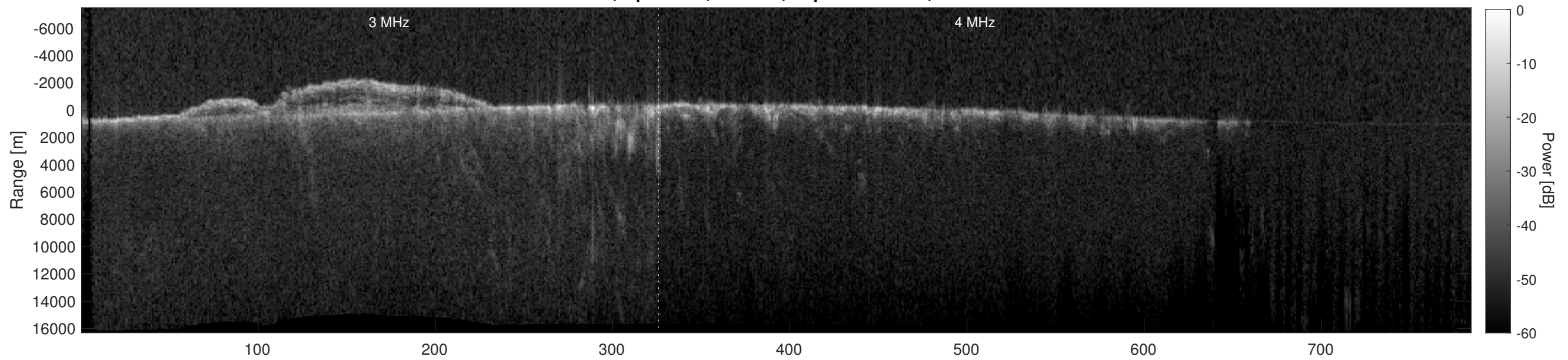
Orbit 9571, Depth-Corrected Cluttergram
