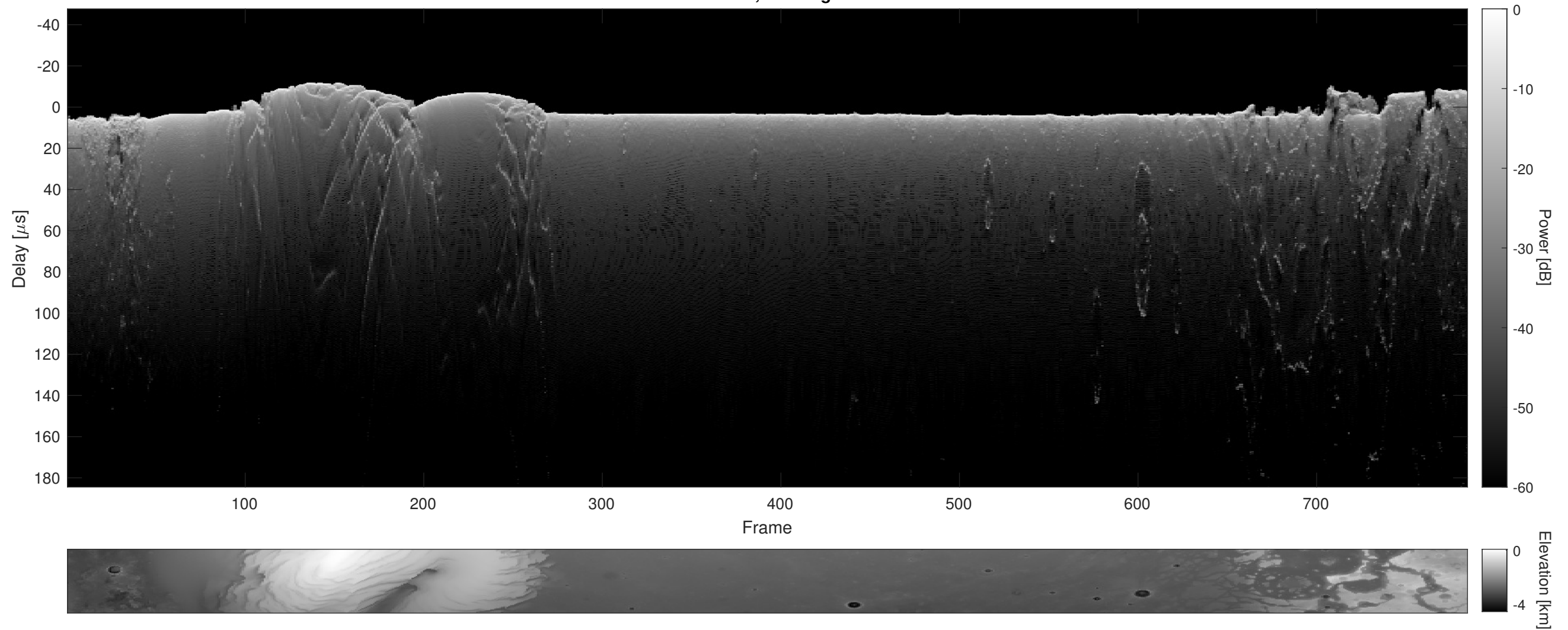
Orbit 9572, Cluttergram
