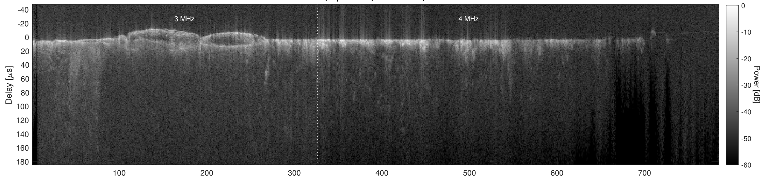
Orbit 9572, Cluttergram
