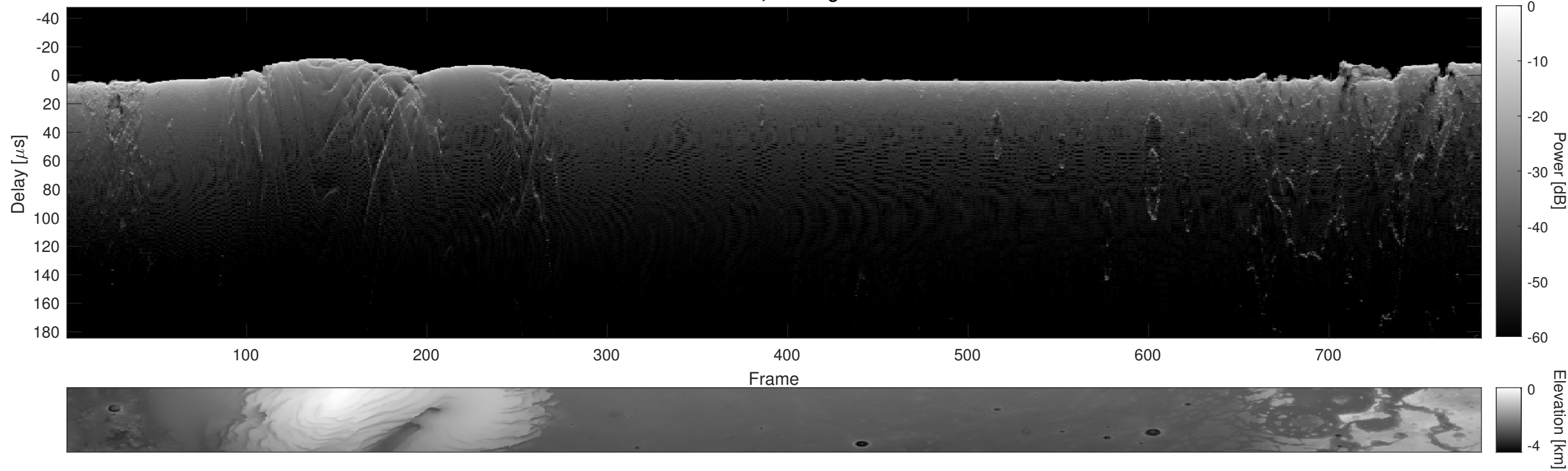
Orbit 9572, Cluttergram
