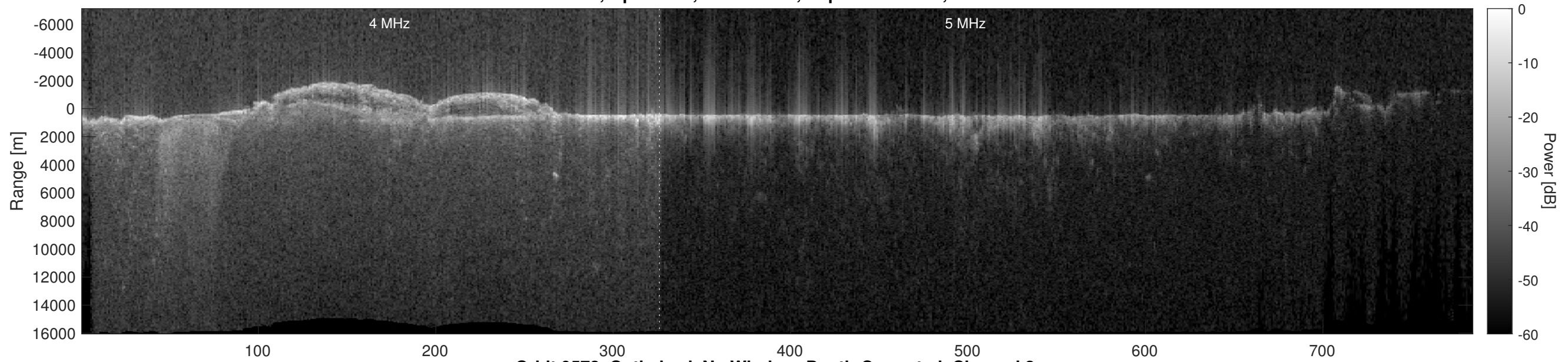
Orbit 9572, Optimized, No Window, Depth-Corrected, Channel 2
