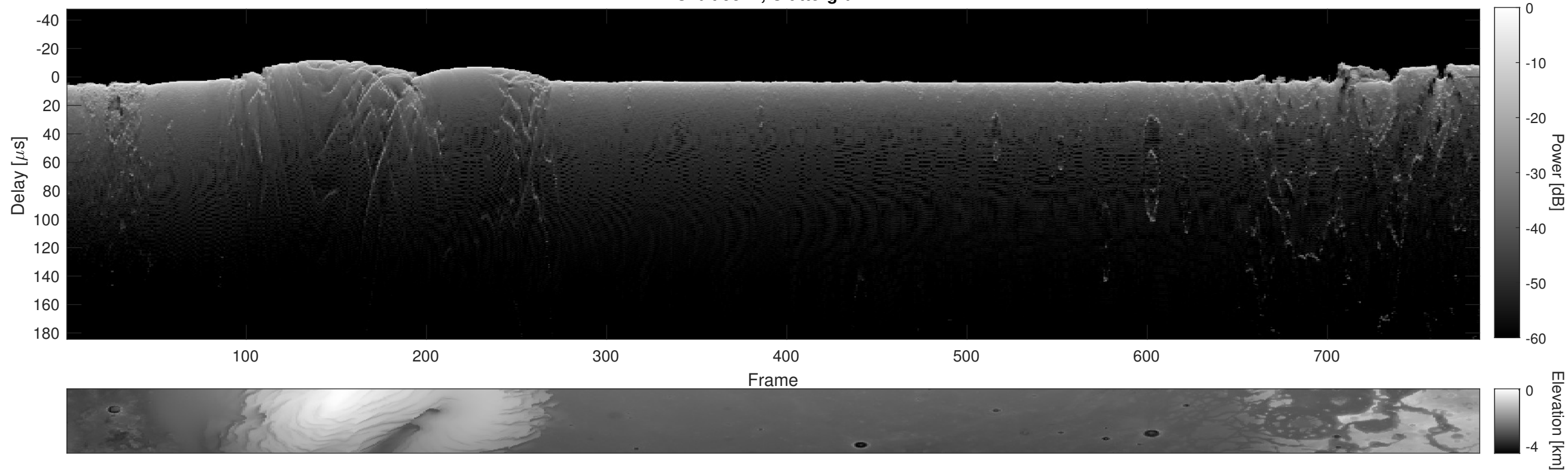
Orbit 9572, Cluttergram
