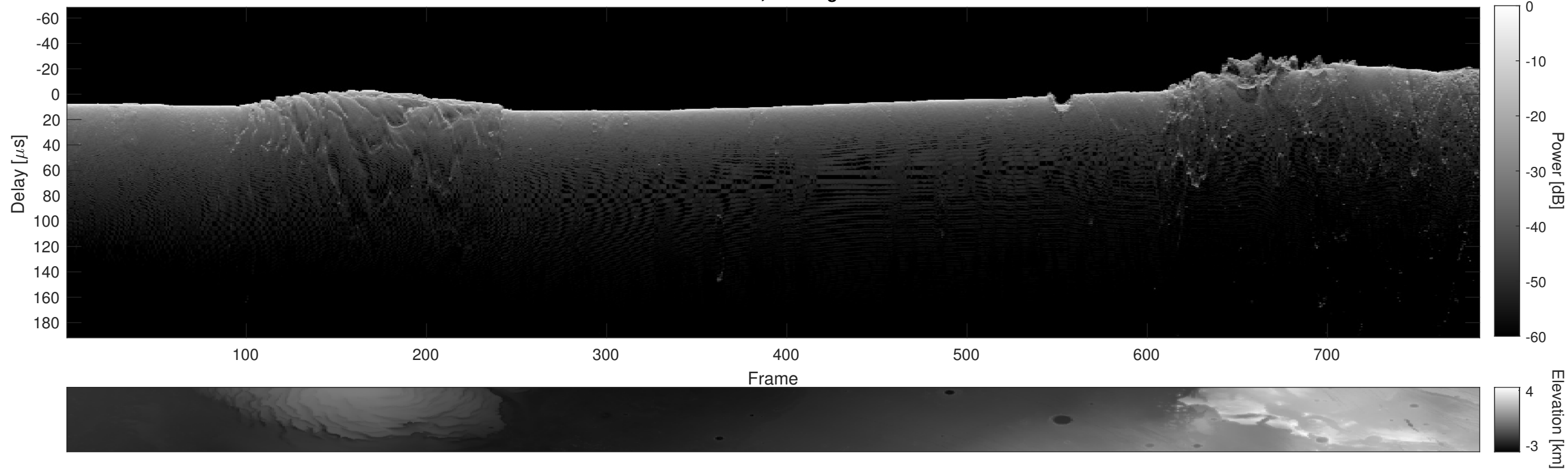
Orbit 9573, Cluttergram
