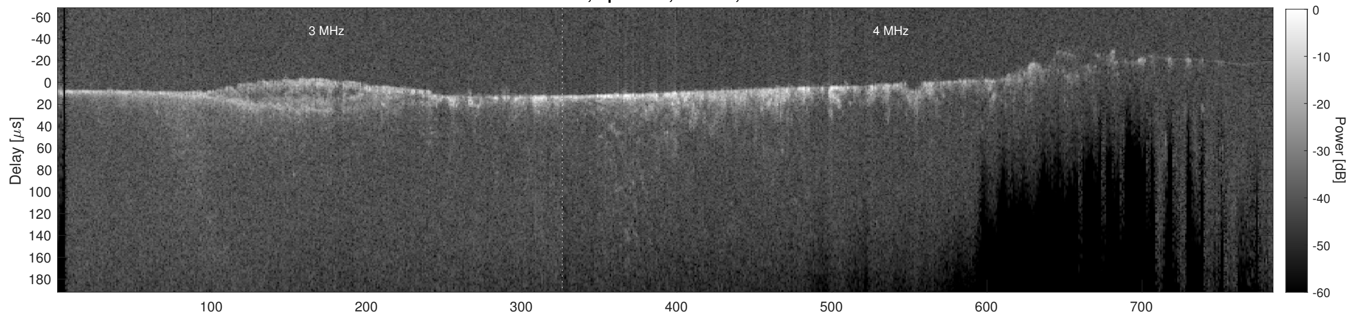
Orbit 9573, Cluttergram
