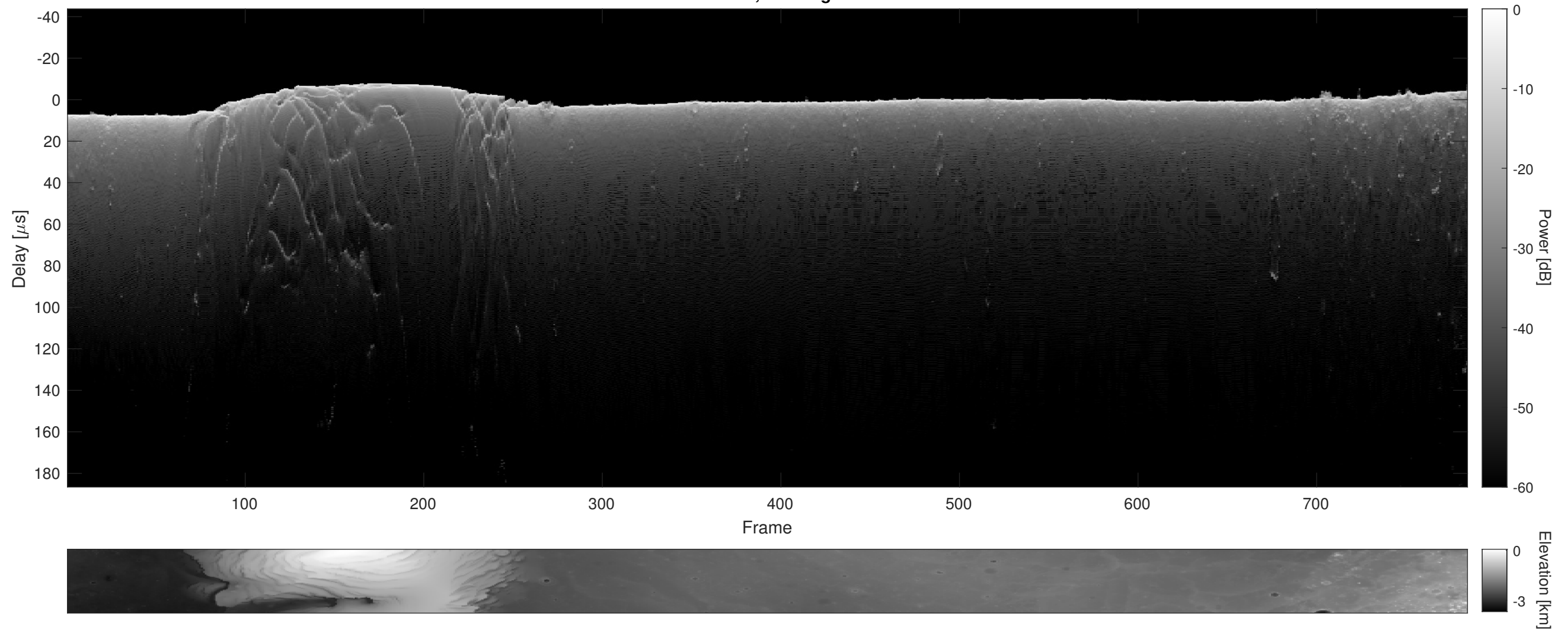
Orbit 9575, Cluttergram
