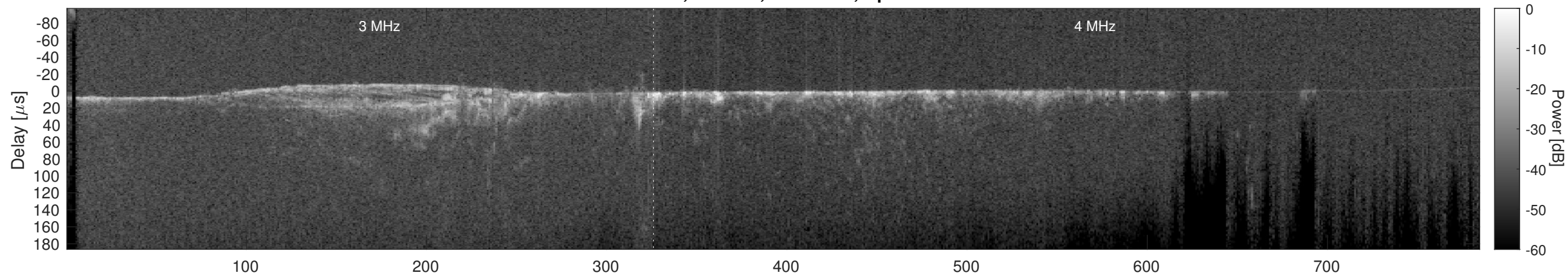
Orbit 9575, Cluttergram
