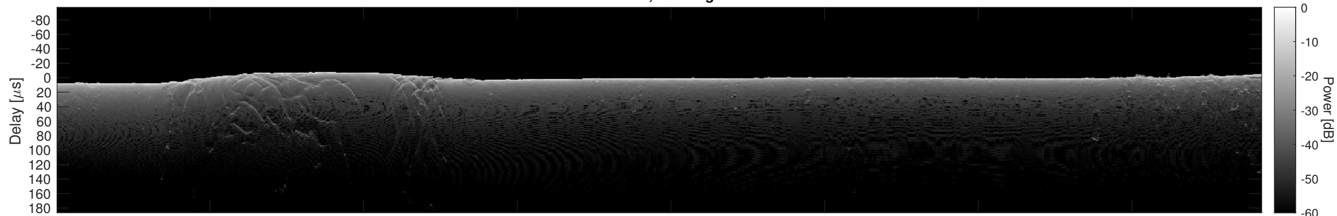
Orbit 9575, Cluttergram
