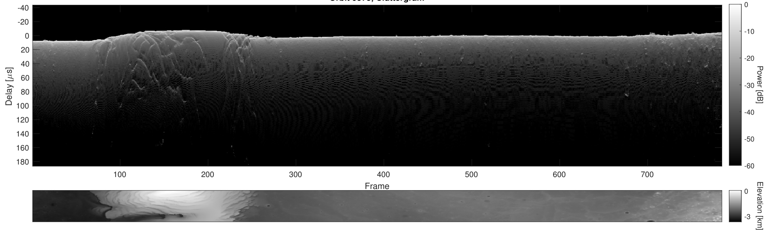
Orbit 9575, Cluttergram
