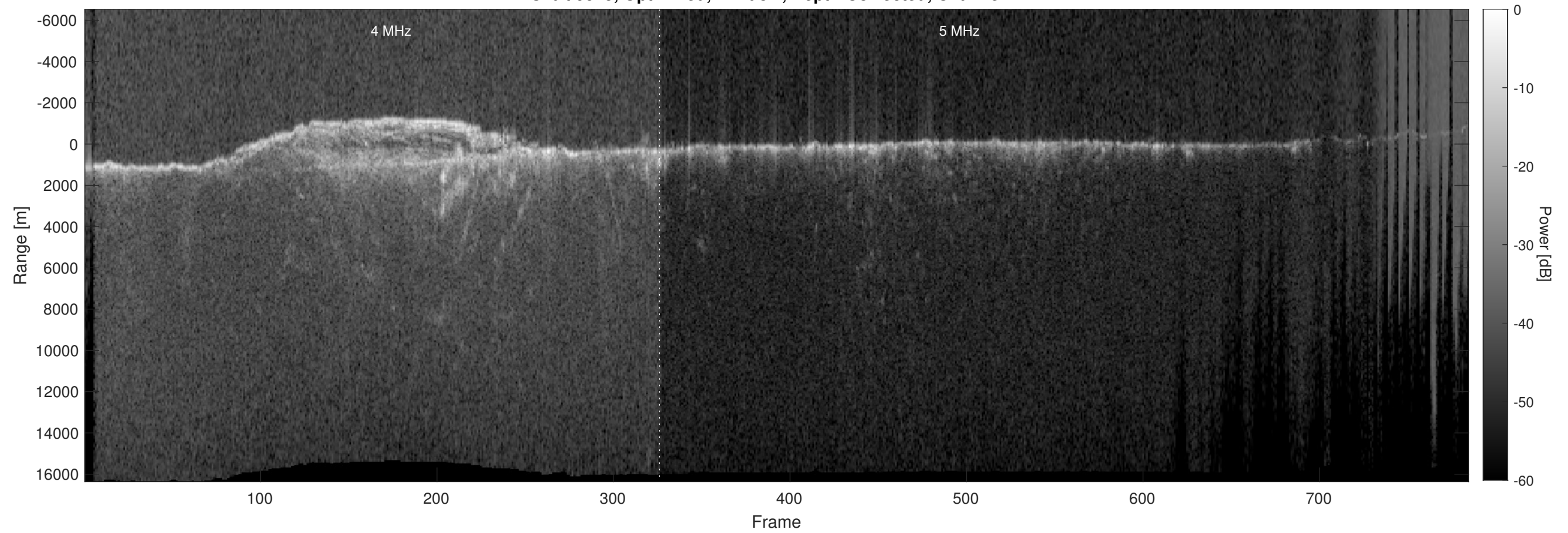
Orbit 9575, Optimized, Window, Depth-Corrected, Channel 2
