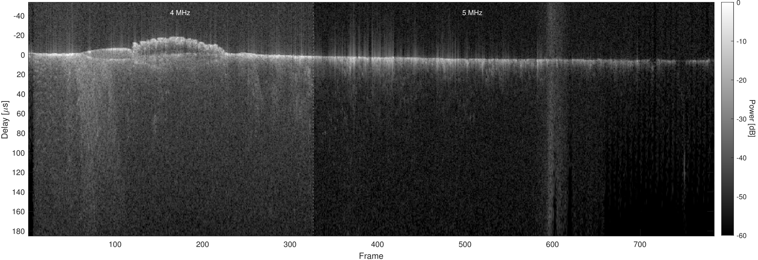
Orbit 9576, Optimized, No Window, Channel 2
