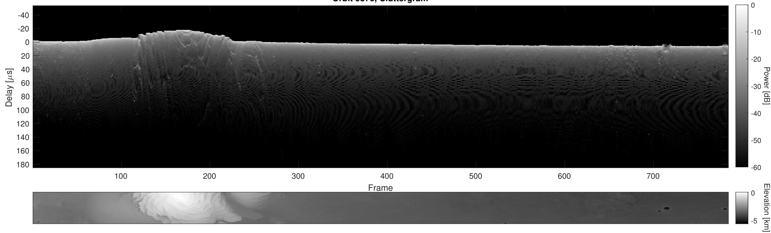
Orbit 9576, Cluttergram
