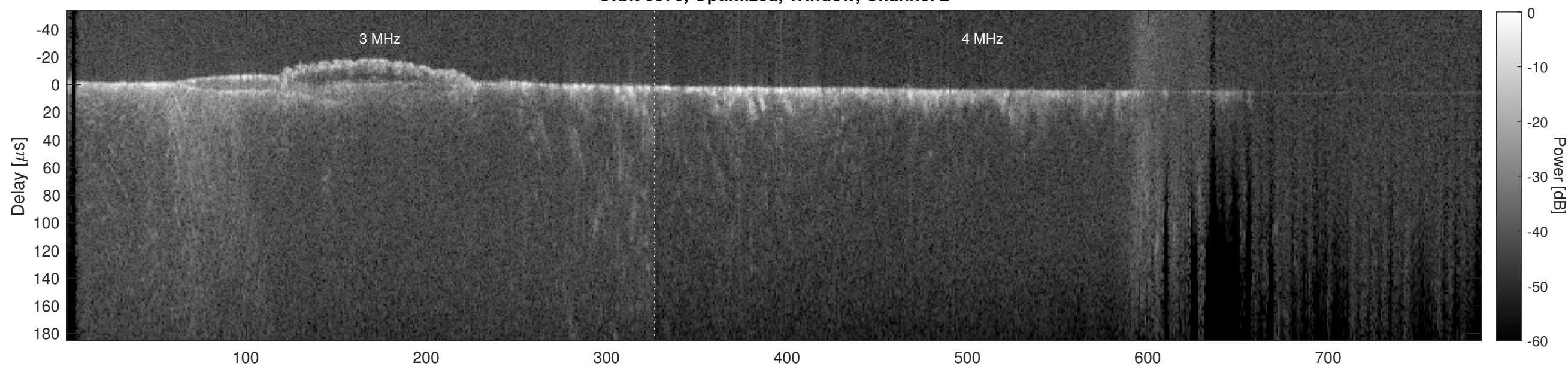
Orbit 9576, Cluttergram
