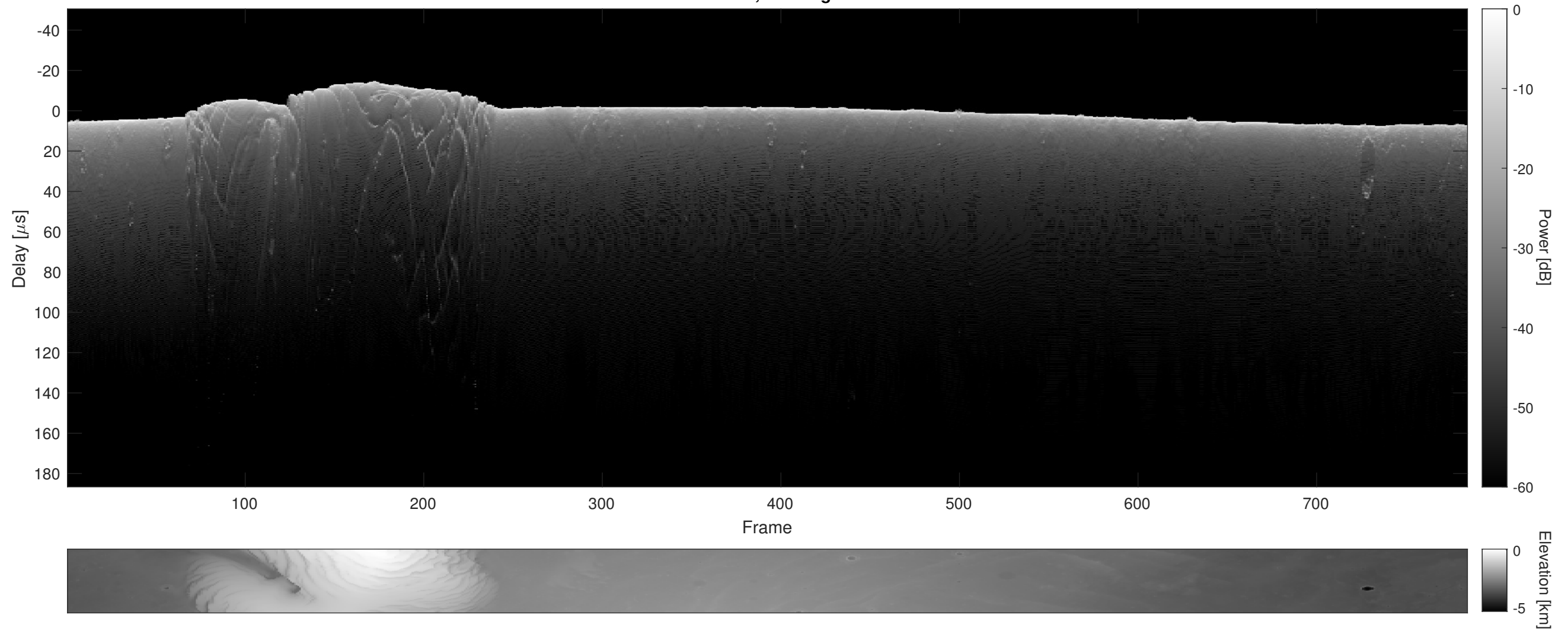
Orbit 9578, Cluttergram
