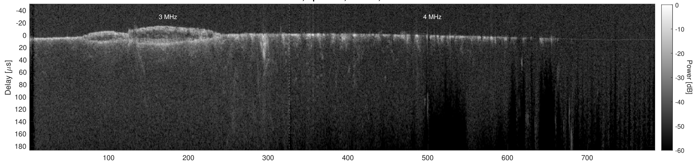
Orbit 9578, Cluttergram
