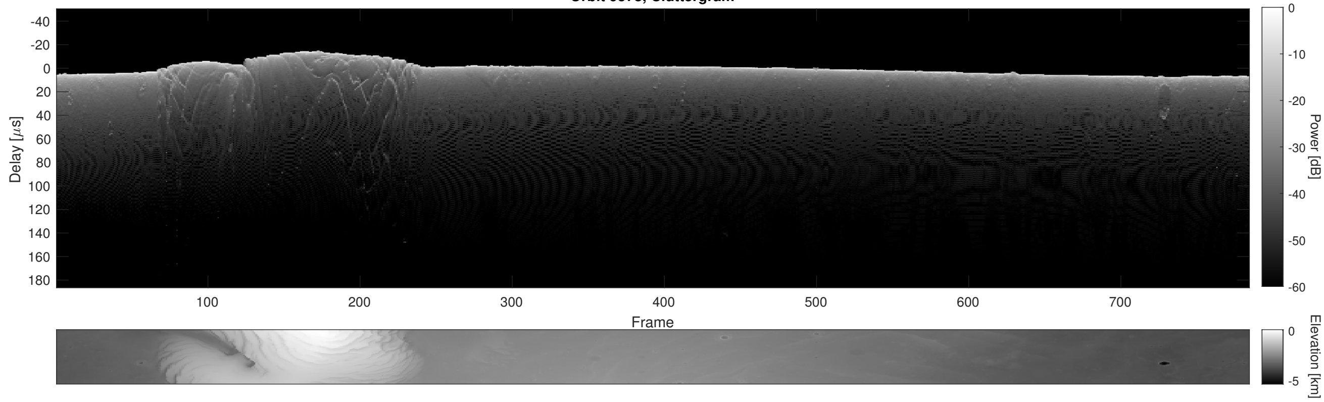
Orbit 9578, Cluttergram
