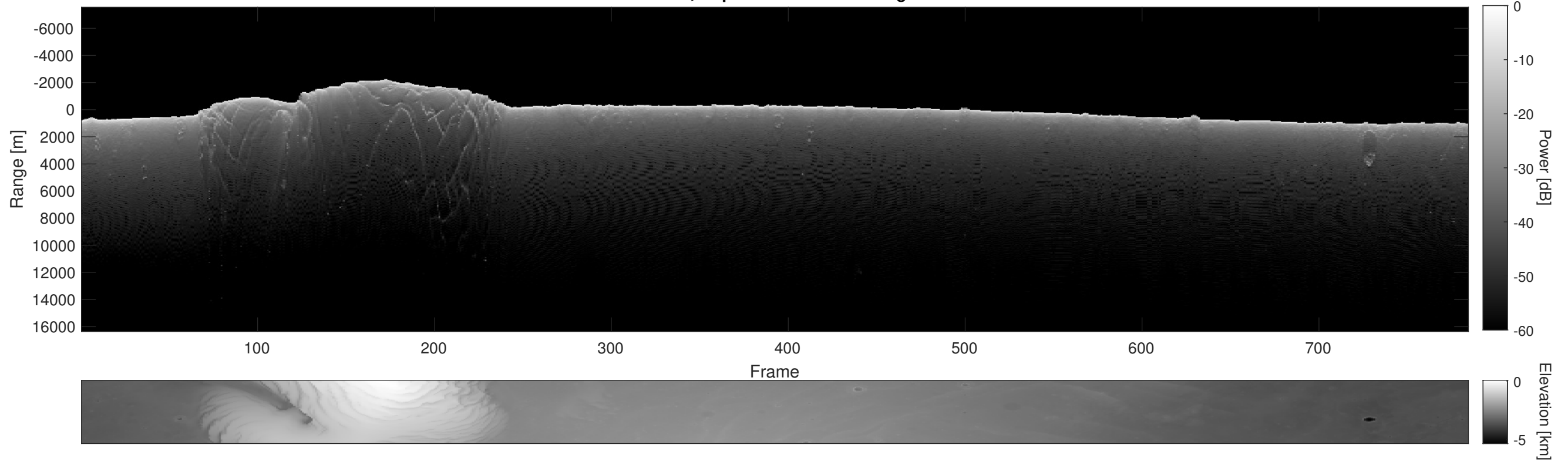
Orbit 9578, Depth-Corrected Cluttergram
