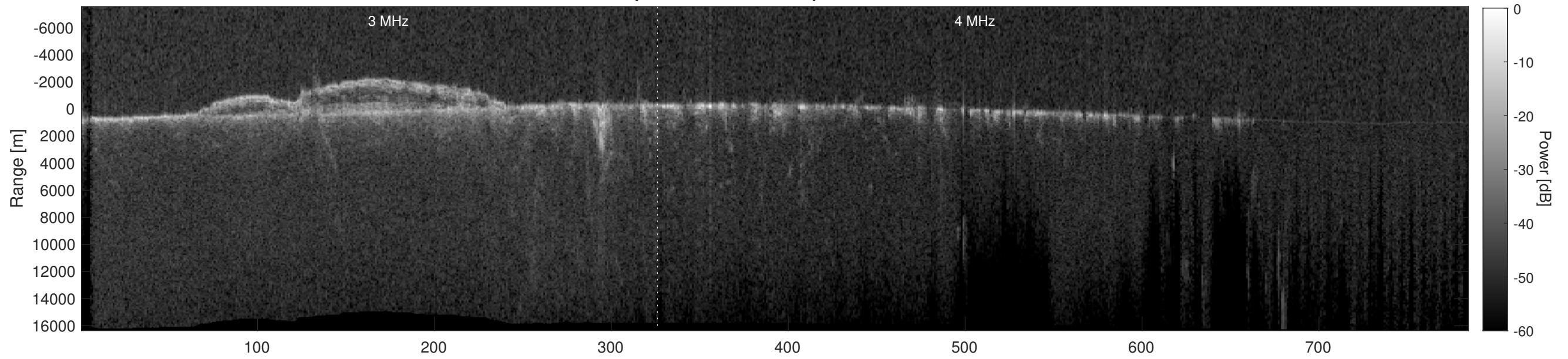
Orbit 9578, Depth-Corrected Cluttergram
