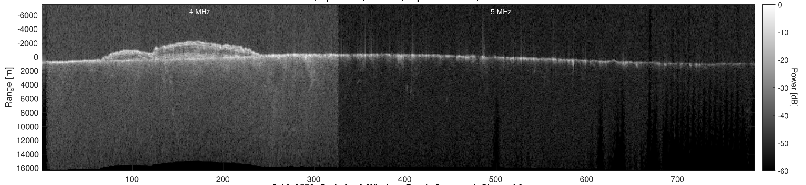
Orbit 9578, Optimized, Window, Depth-Corrected, Channel 2
