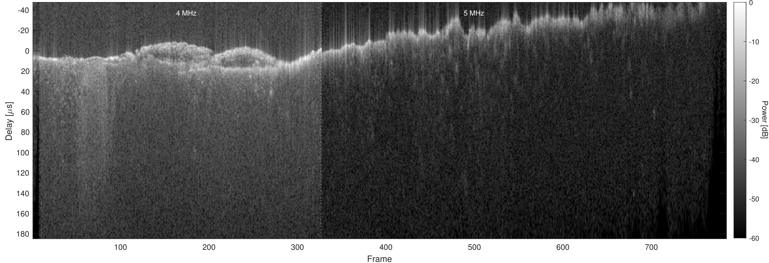
Orbit 9579, Chapman, No Window, Channel 2
