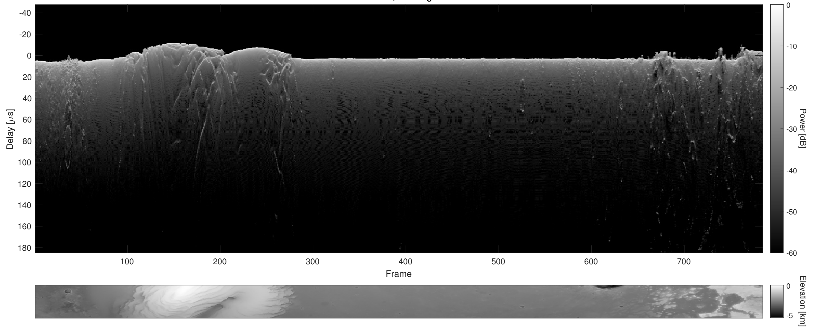
Orbit 9579, Cluttergram
