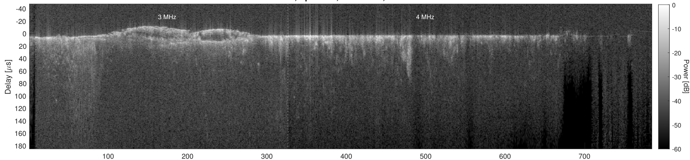
Orbit 9579, Cluttergram
