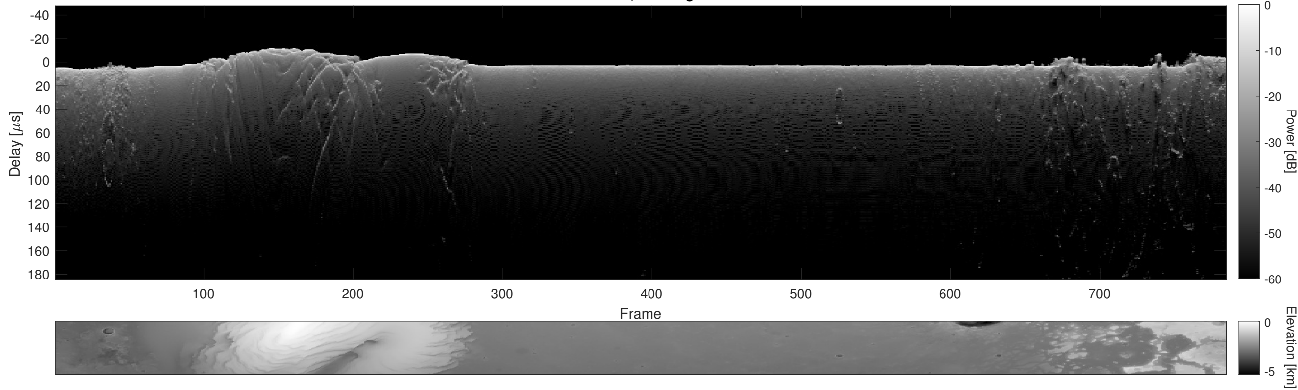
Orbit 9579, Cluttergram
