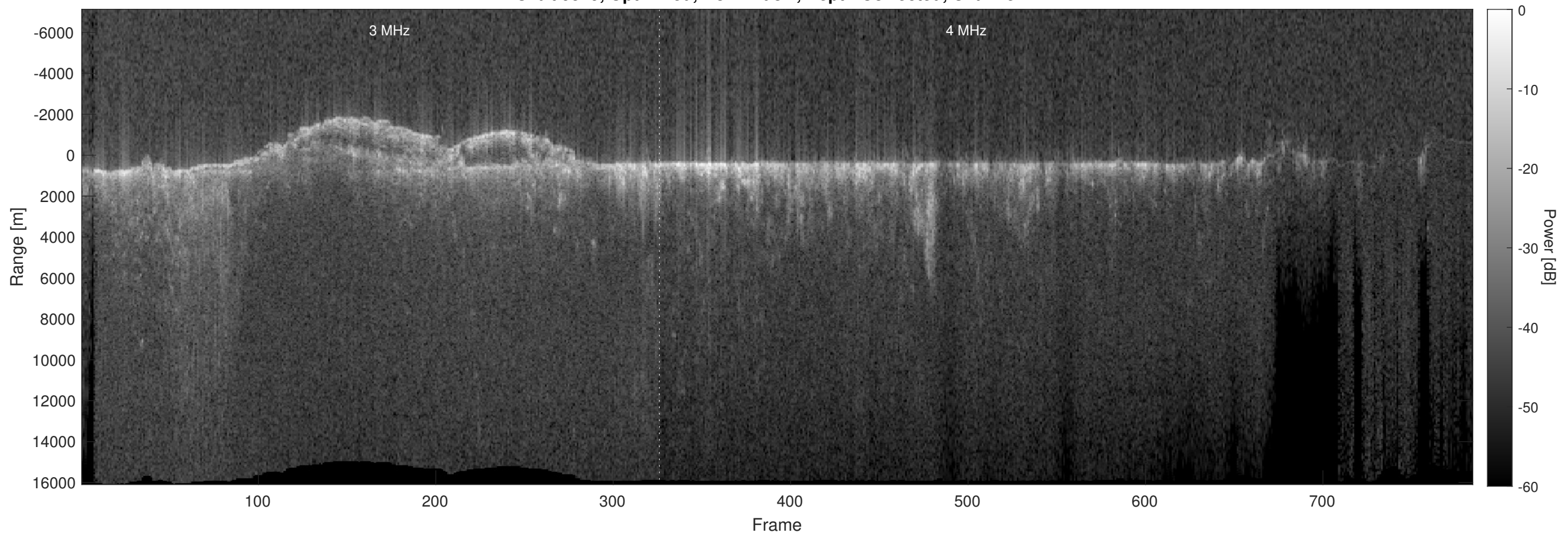
Orbit 9579, Optimized, No Window, Depth-Corrected, Channel 2
