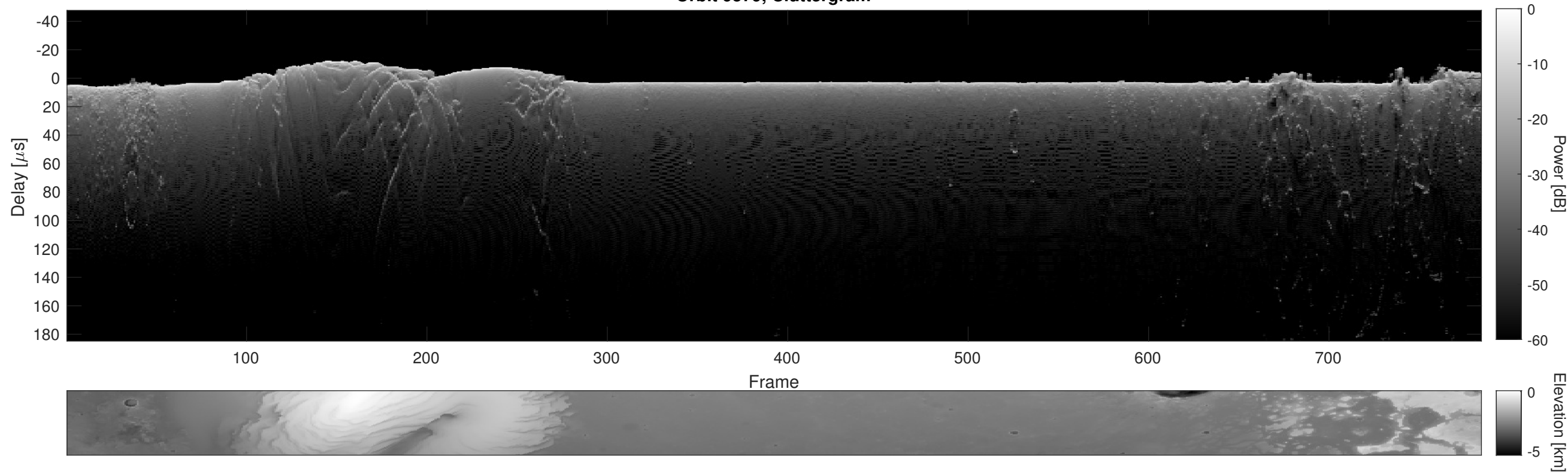
Orbit 9579, Cluttergram
