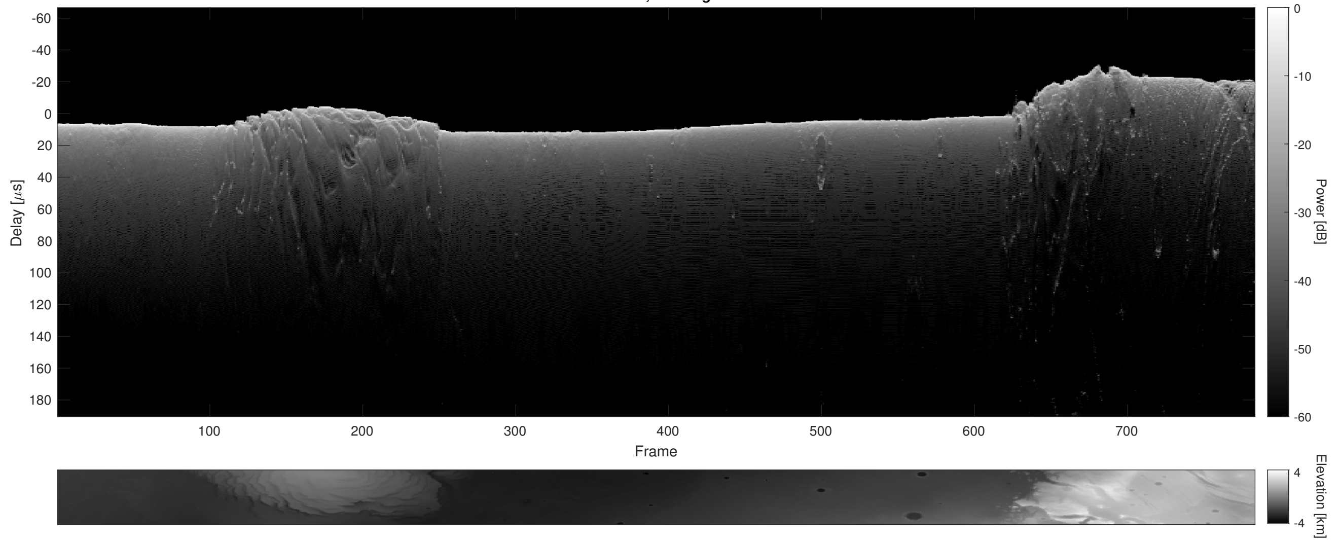
Orbit 9580, Cluttergram
