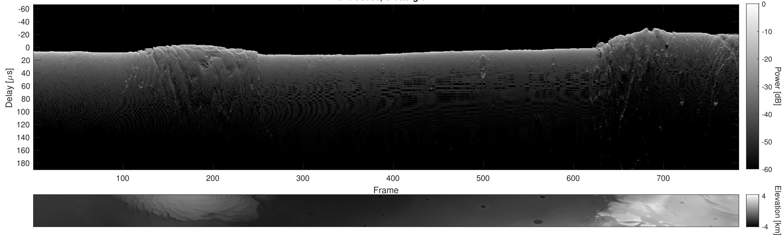
Orbit 9580, Cluttergram
