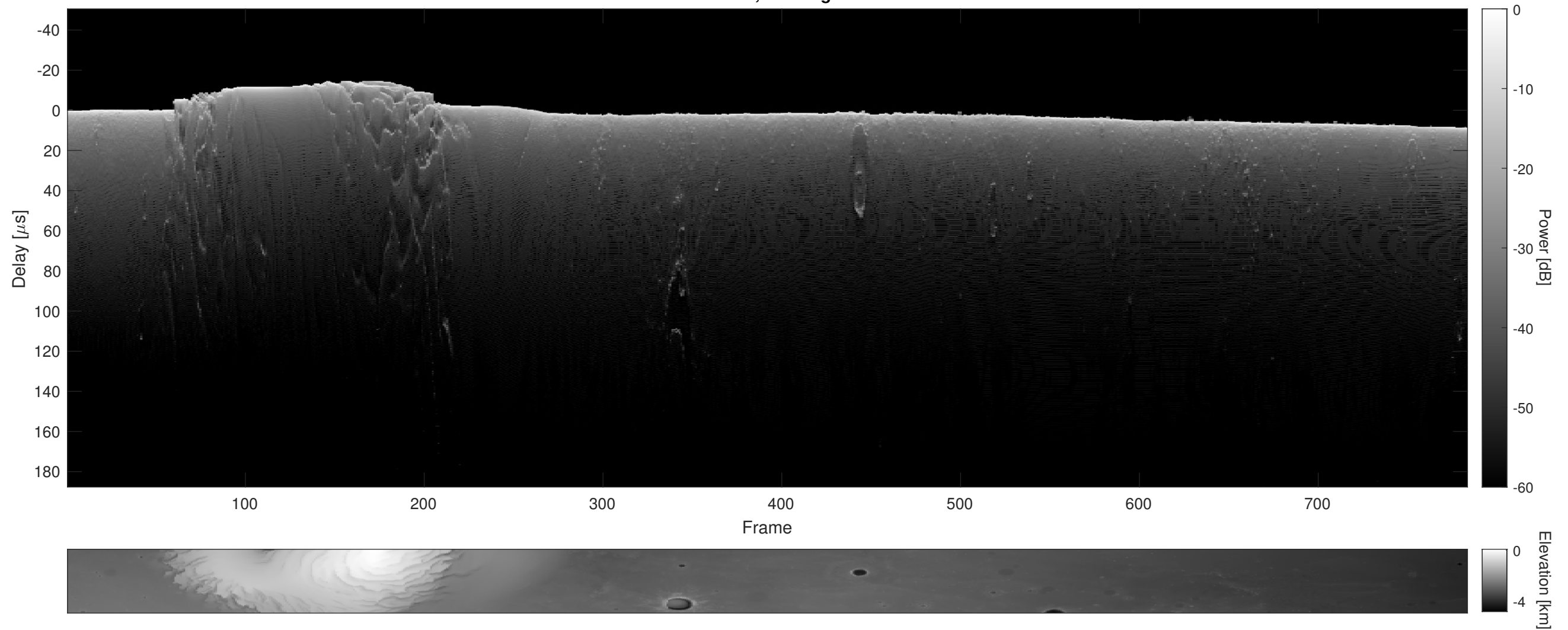
Orbit 9581, Cluttergram
