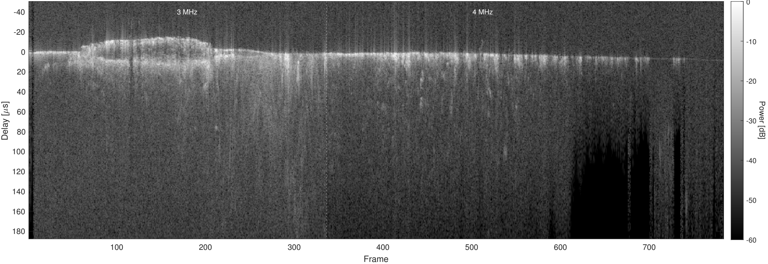
Orbit 9581, Optimized, No Window, Channel 2
