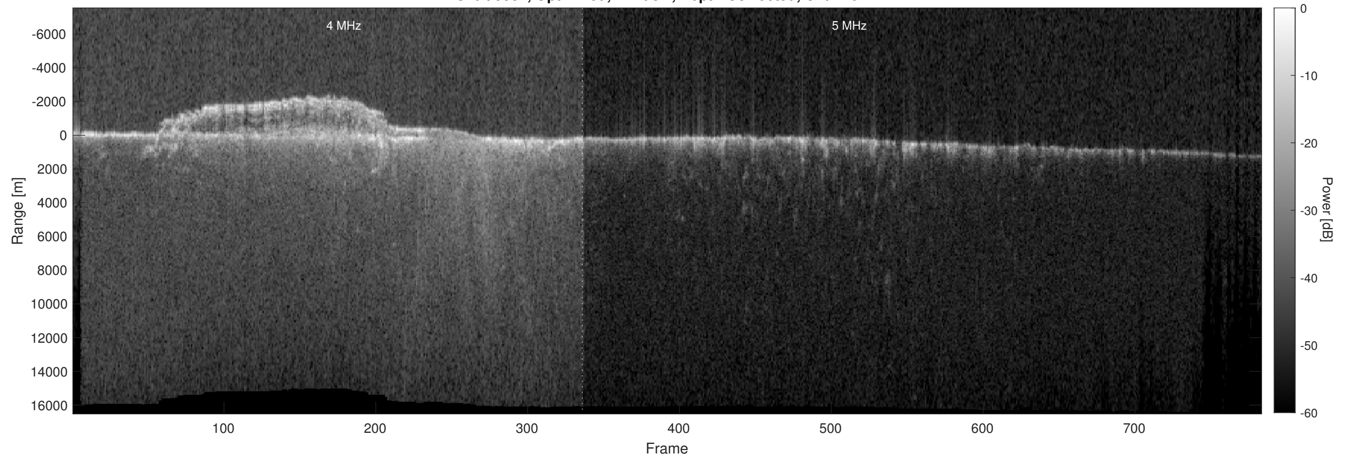
Orbit 9581, Optimized, Window, Depth-Corrected, Channel 2
