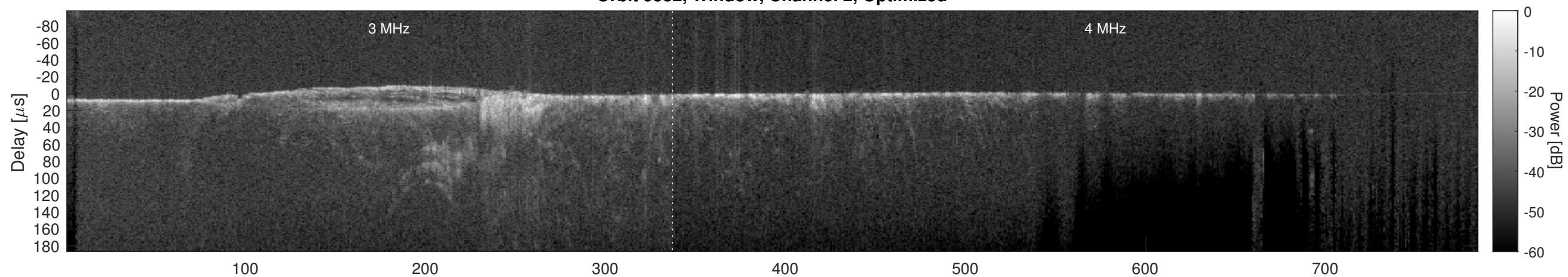
Orbit 9582, Cluttergram
