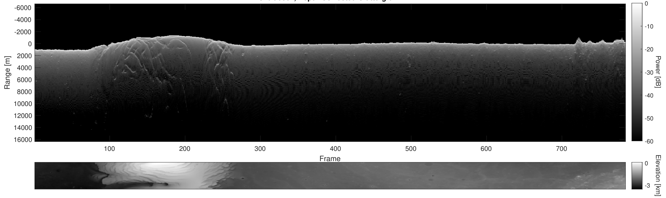
Orbit 9582, Depth-Corrected Cluttergram
