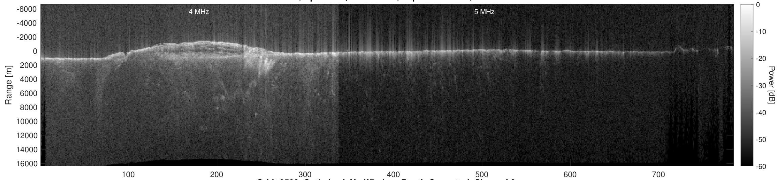
Orbit 9582, Optimized, No Window, Depth-Corrected, Channel 2
