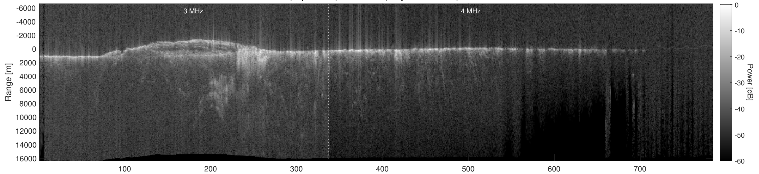
Orbit 9582, Depth-Corrected Cluttergram
