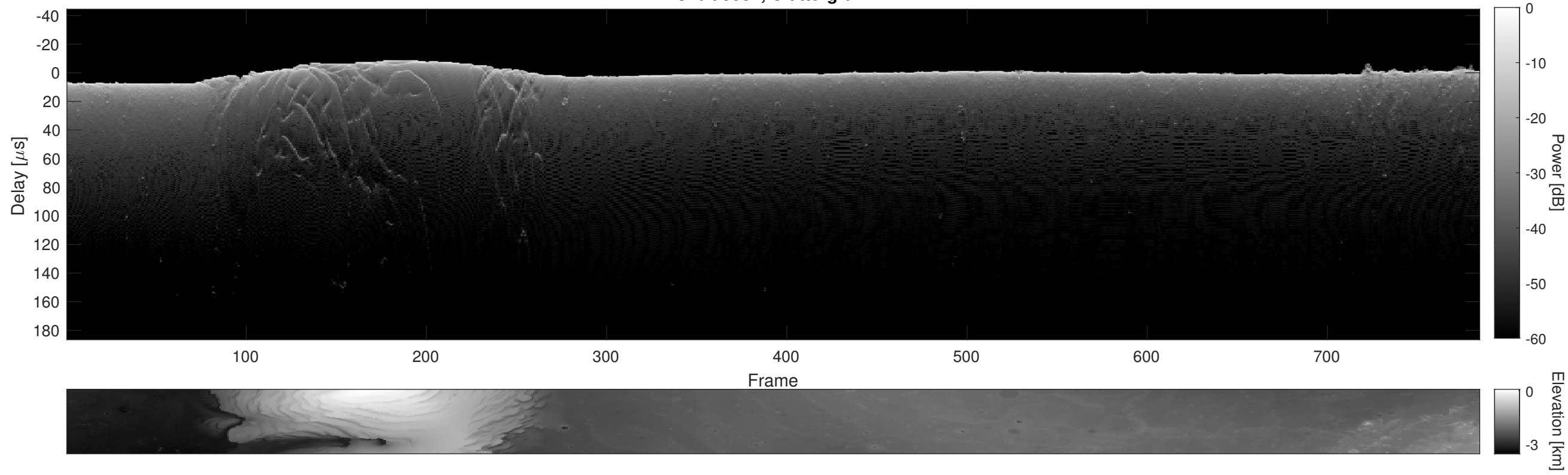
Orbit 9582, Cluttergram
