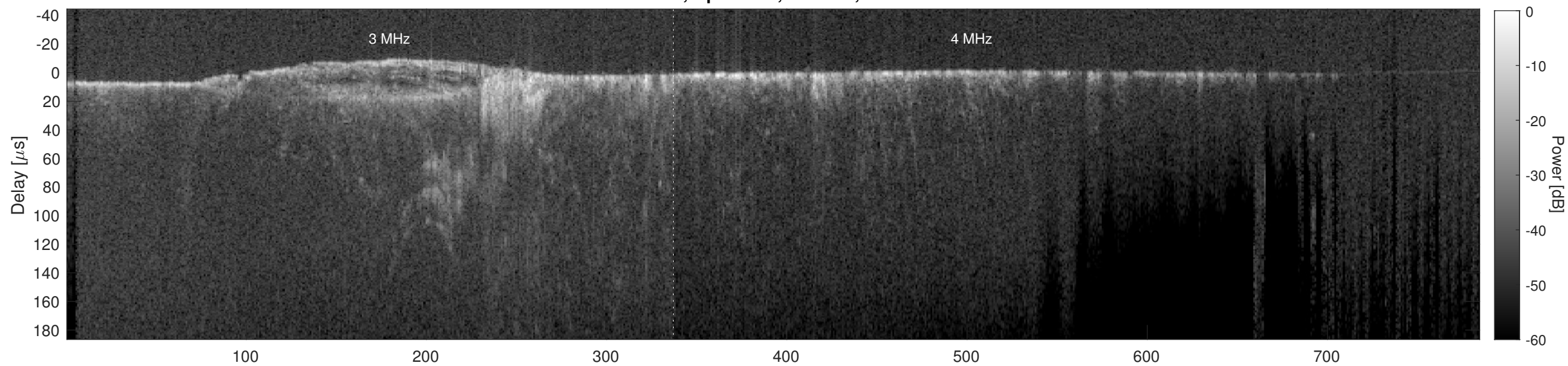
Orbit 9582, Cluttergram
