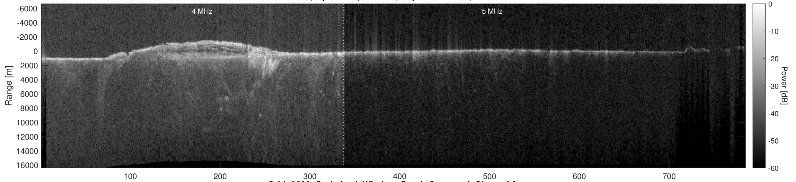
Orbit 9582, Optimized, Window, Depth-Corrected, Channel 2
