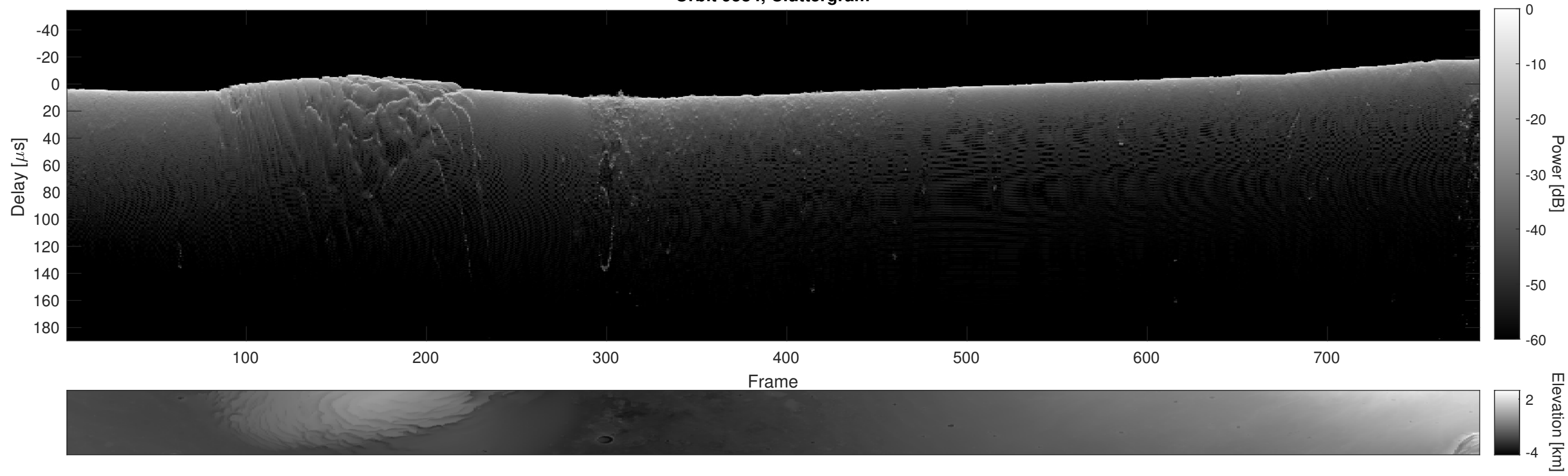
Orbit 9584, Cluttergram
