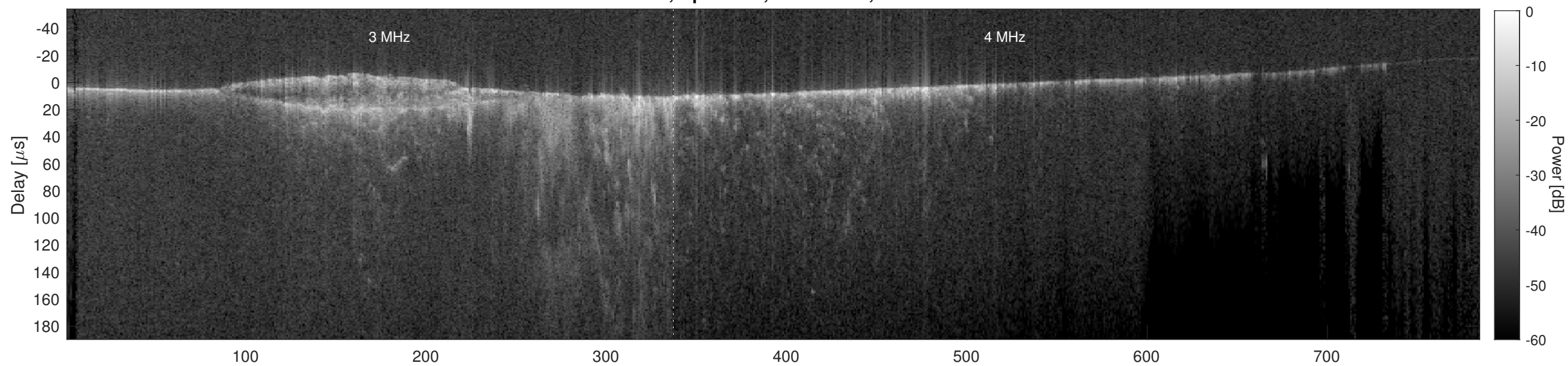
Orbit 9584, Cluttergram
