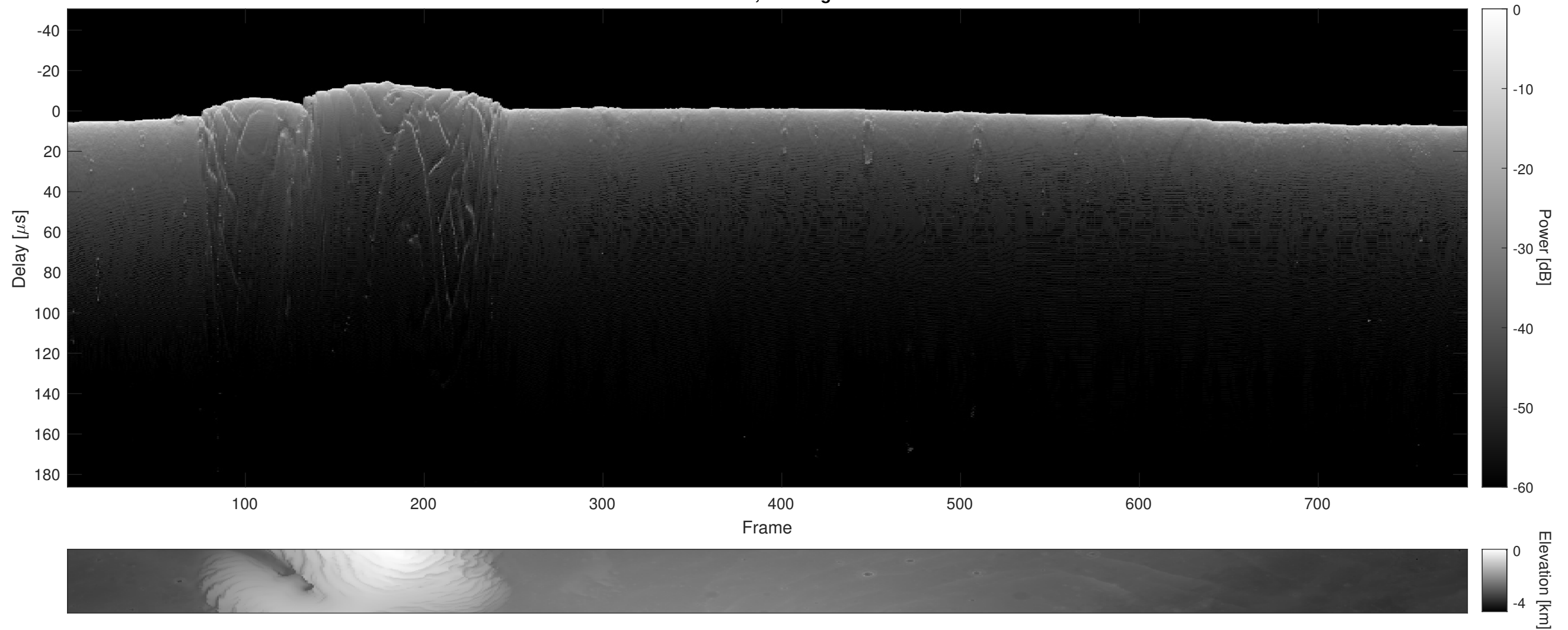
Orbit 9585, Cluttergram
